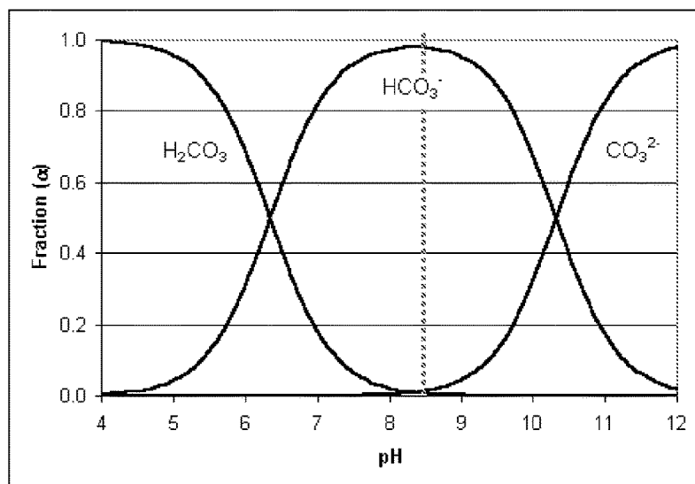
Graph 2-3: Carbonate species as a function of pH
