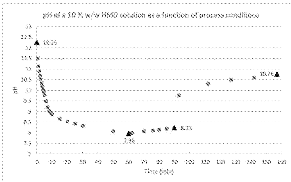
Graph 1-3: pH as a function of process conditions, refer to Table 1-1 above.
