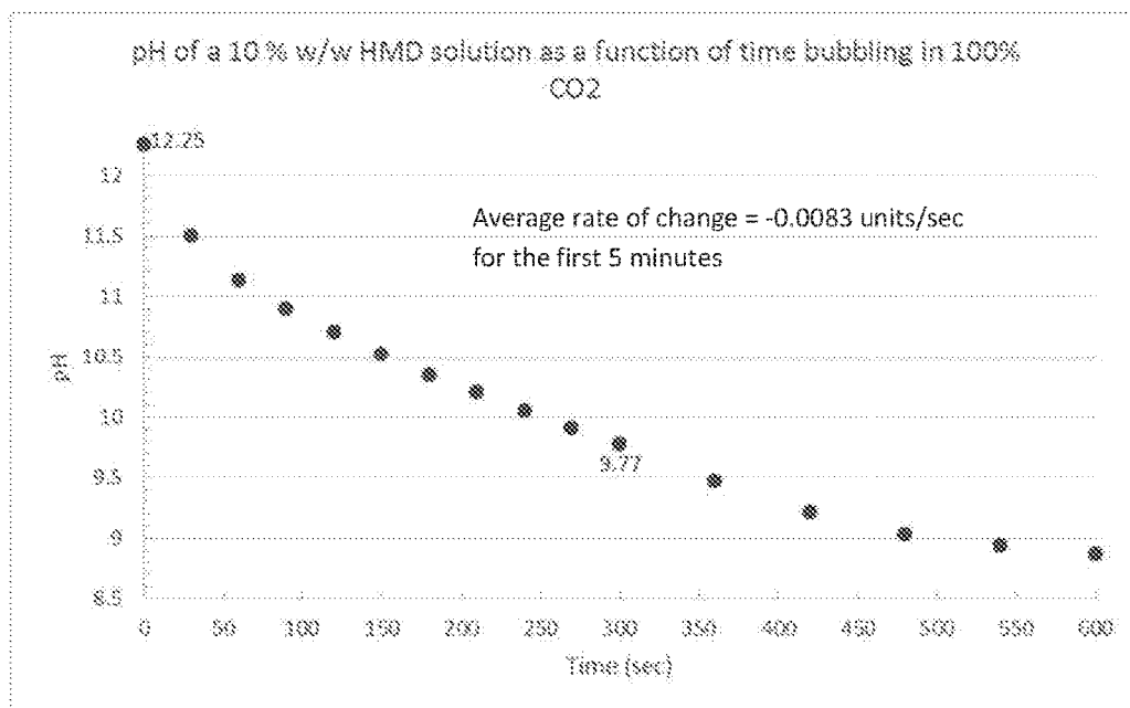
Graph 1-2: pH as a function of time bubbling in CO 2 first 10 minutes.
