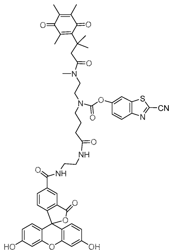
5684: 2-cyanobenzo[d]thiazol-6-yl (4-((2-(3',6'-dihydroxy-3-oxo-3H-spiro[isobenzofuran-1,9'-xanthene]-5-carboxamido)ethyl)amino)-4-oxobutyl)(2-(N,3-dimethyl-3-(2,4,5-trimethyl-3,6-dioxocyclohexa-1,4-dien-1-yl)butanamido)ethyl)carbamate;
