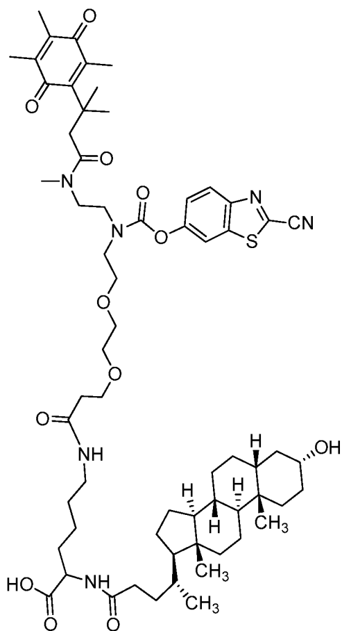
5647: 8-(((2-cyanobenzo[d]thiazol-6-yl)oxy)carbonyl)-23-((R)-4-((3R,5R,8R,9S,10S,13R,14S,17R)-3-hydroxy-10,13-dimethylhexadecahydro-1H-cyclopenta[a]phenanthren-17-yl)pentanamido)-2,5-dimethyl-4,17-dioxo-2-(2,4,5-trimethyl-3,6-dioxocyclohexa-1,4-dien-1-yl)-11,14-dioxa-5,8,18-triazatetracosan-24-oic acid;
