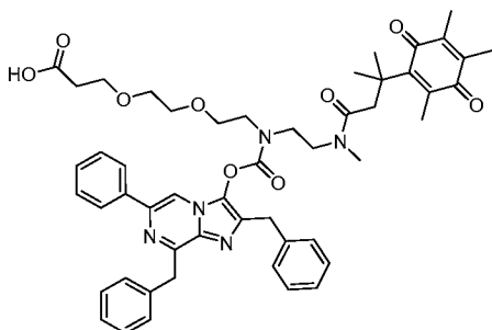
PBI 5471
