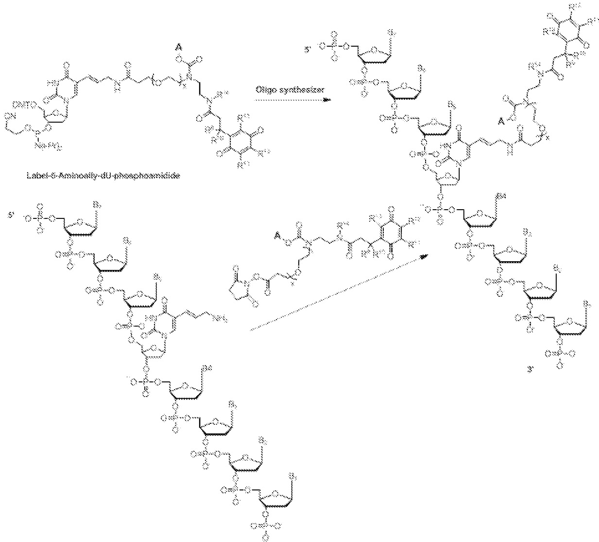
Scheme 1
