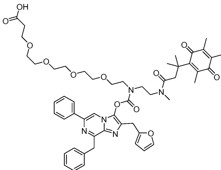
PBI 5463
