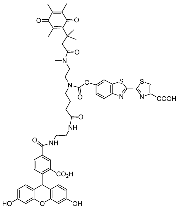
5824: 2-(6-(((4-((2-(3-carboxy-4-(3,6-dihydroxy-9H-xanthen-9-yl)benzamido)ethyl)amino)-4-oxobutyl)(2-(N,3-dimethyl-3-(2,4,5-trimethyl-3,6-dioxocyclohexa-1,4-dien-1-yl)butanamide)ethyl)carbamoyl)oxy)benzo[d]thiazol-2-yl)thiazole-4-carboxylic acid;
