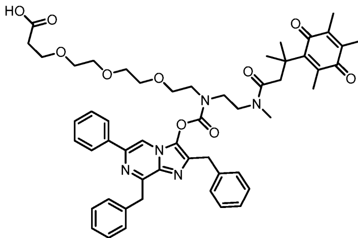
5470: 13-(((2,8-dibenzyl-6-phenylimidazo[1,2-a]pyrazin-3-yl)oxy)carbonyl)-16,19-dimethyl-17-oxo-19-(2,4,5-trimethyl-3,6-dioxocyclohexa-1,4-dien-1-yl)-4,7,10-trioxa-13,16-diazaicosan-1-oic acid;
