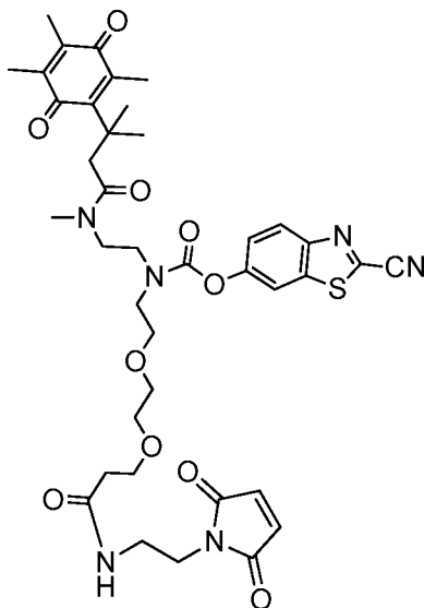
5915: 2-cyanobenzo[d]thiazol-6-yl (2-(N,3-dimethyl-3-(2,4,5-trimethyl-3,6-dioxocyclohexa-1,4-dien-1-yl)butanamido)ethyl)(2-(2-(3-((2-(2,5-dioxo-2,5-dihydro-1H-pyrrol-1-yl)ethyl)amino)-3-oxopropoxy)ethoxy)ethyl)carbamate;
