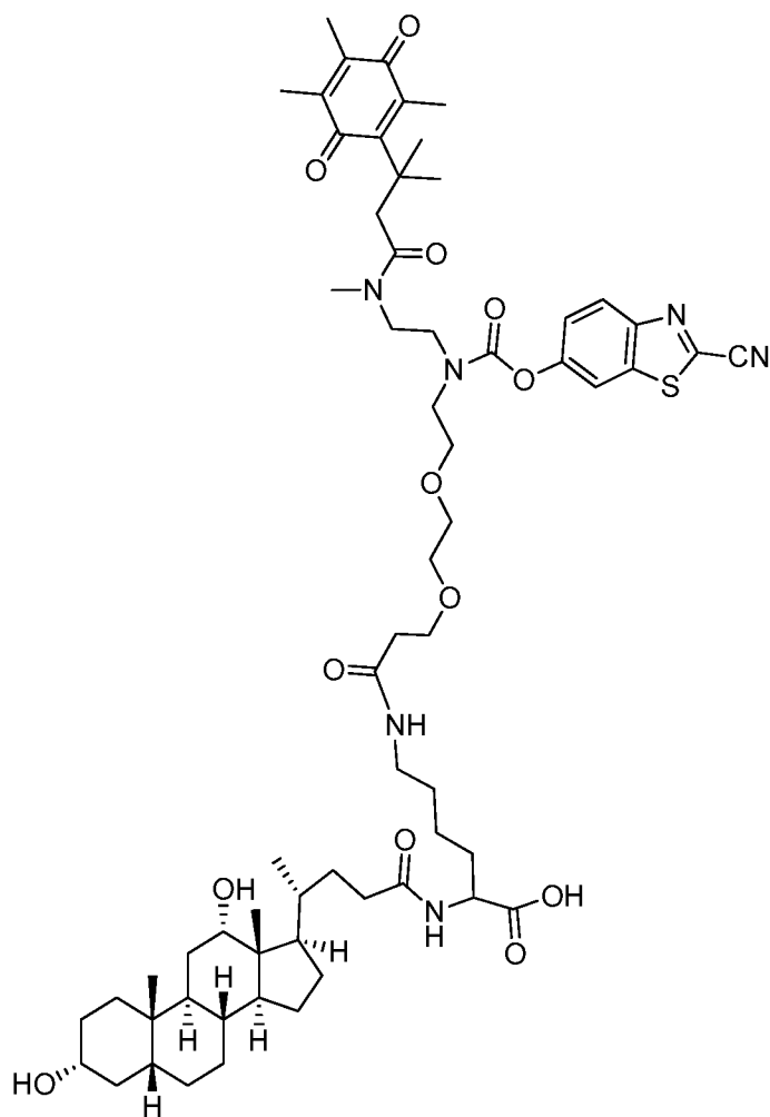
5625: 8-(((2-cyanobenzo[d]thiazol-6-yl)oxy)carbonyl)-23-((R)-4-((3R,5R,8R,9S,10S,12S,13R,14S,17R)-3,12-dihydroxy-10,13-dimethylhexadecahydro-1H-cyclopenta[a]phenanthren-17-yl)pentanamido)-2,5-dimethyl-4,17-dioxo-2-(2,4,5-trimethyl-3,6-dioxocyclohexa-1,4-dien-1-yl)-11,14-dioxo-5,8,18-triazatetracosan-24-oic acid;
