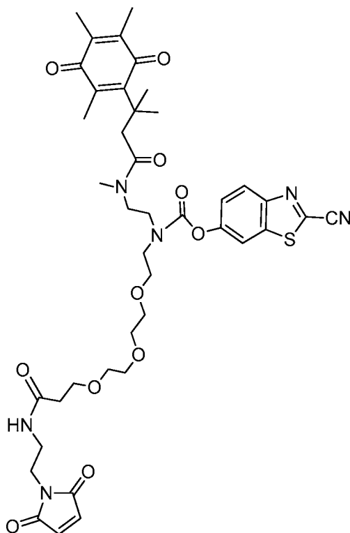
5915: 2-cyanobenzo[d]thiazol-6-yl (2-(N,3-dimethyl-3-(2,4,5-trimethyl-3,6-dioxocyclohexa-1,4-dien-1-yl)butanamido)ethyl)(2-(2-(3-((2-(2,5-dioxo-2,5-dihydro-1H-pyrrol-1-yl)ethyl)amino)-3-oxopropoxy)ethoxy)ethyl)carbamate;
