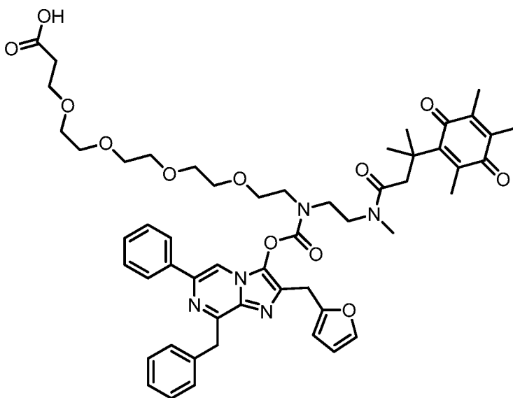
5463: 16-(((8-benzyl-2-(furan-2-ylmethyl)-6-phenylimidazo[1,2-a]pyrazin-3-yl)oxy)carbonyl)-19,22-dimethyl-20-oxo-22-(2,4,5-trimethyl-3,6-dioxocyclohexa-1,4-dien-1-yl)-4,7,10,13-tetraoxa-16,19-diazatricosan-1-oic acid;
