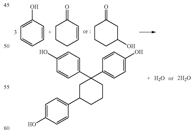
Reaction Formula (1)
