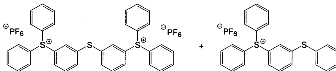
Mixture of two triarylsulfonium hexafluorophosphates above
