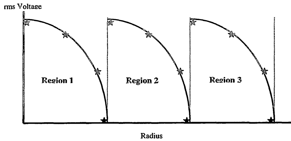
Spatial Voltage Profile for a Converging Electro-active Lens
