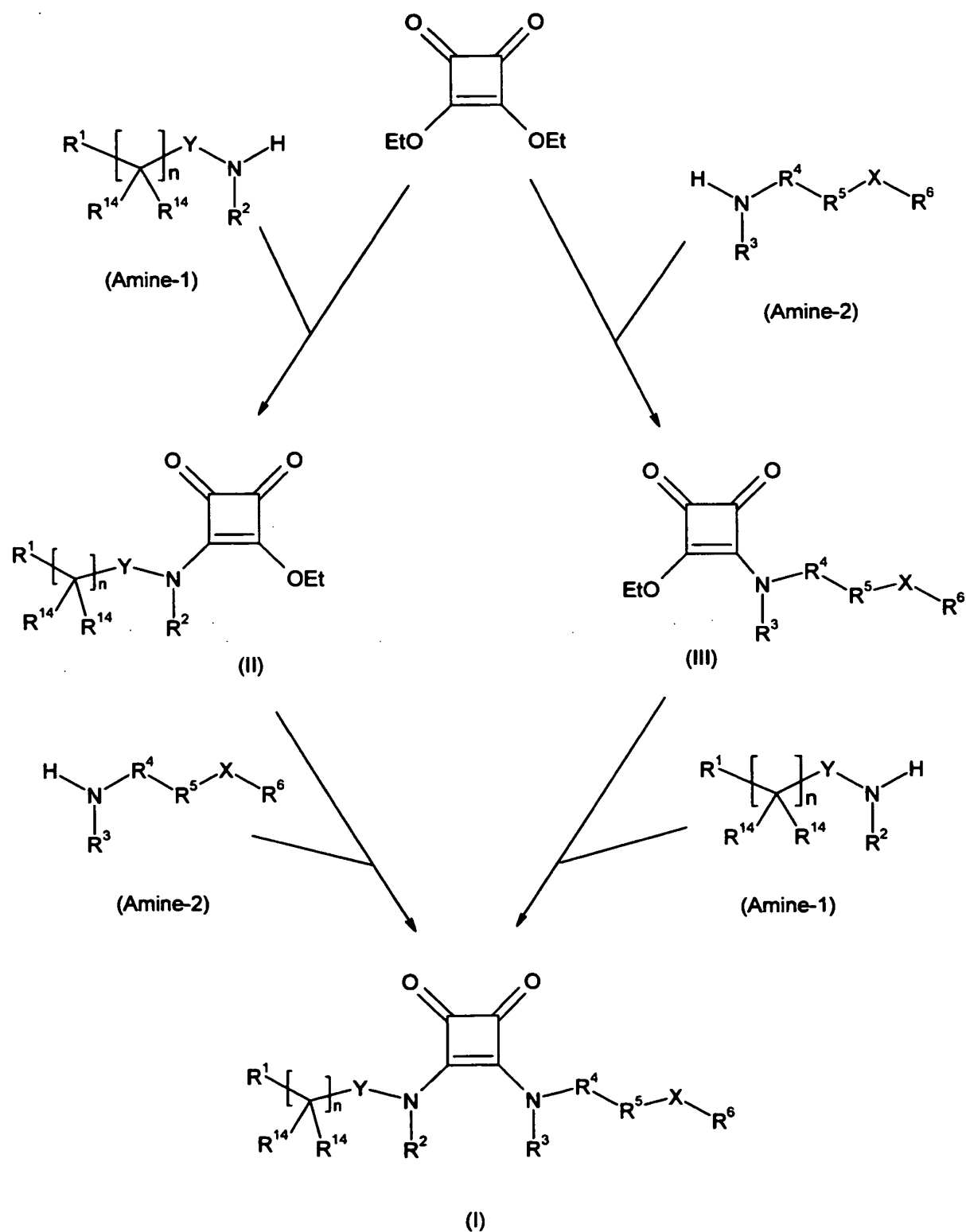
SCHEME 1:
