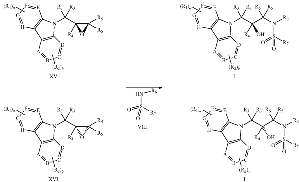
Reaction Scheme V
