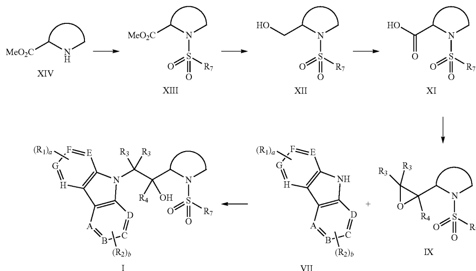
Reaction Scheme IV
