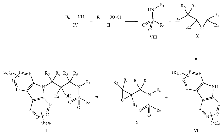
Reaction Scheme III
