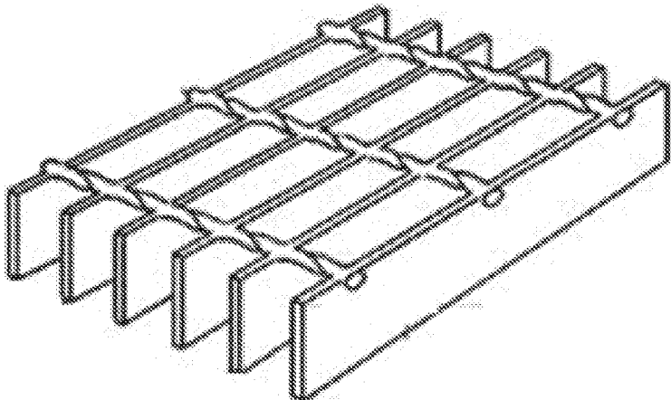
FIG. 3A Crossbar and Bearing grid showing serrated and non serrated bars
