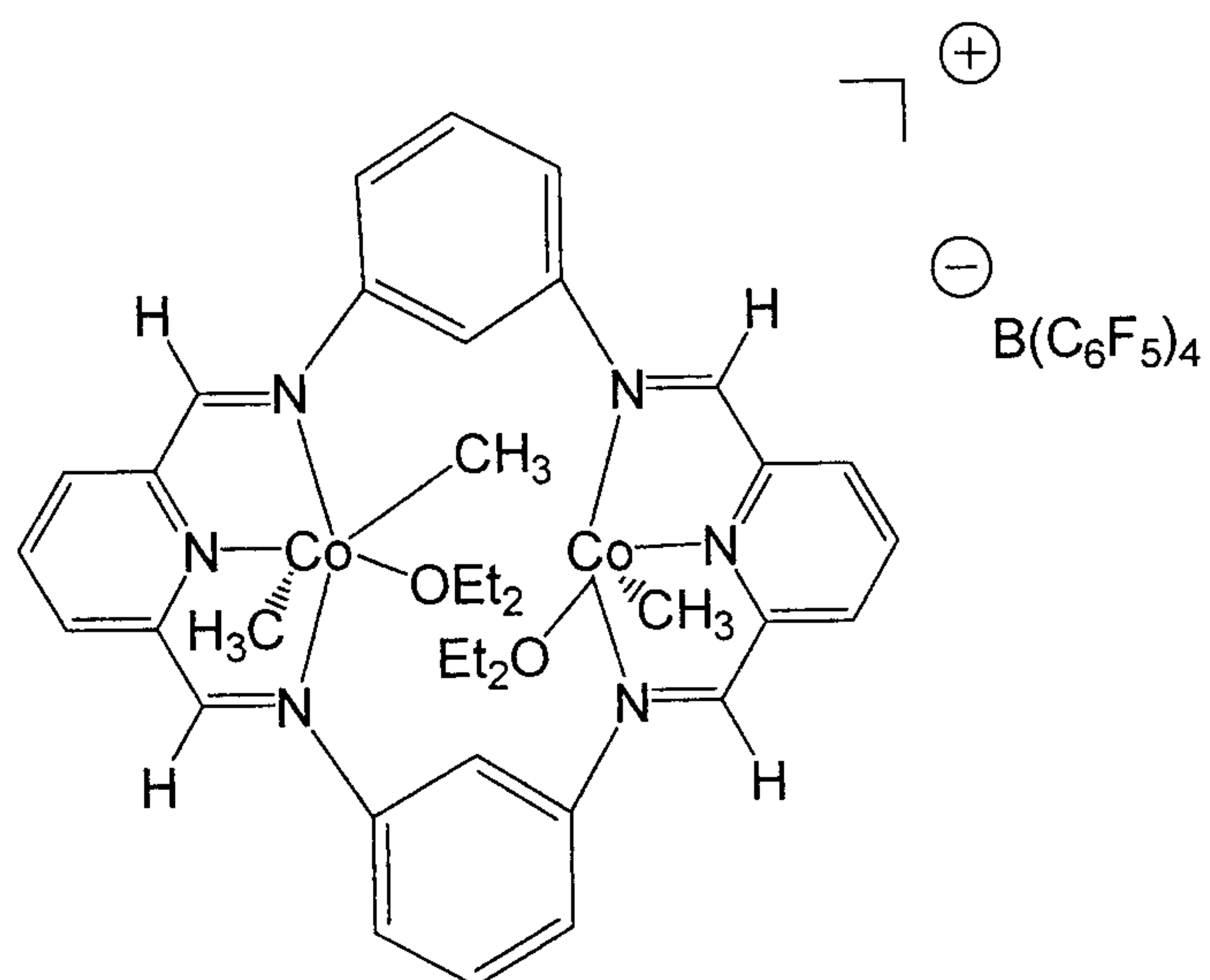
cationic metal-pair complex 4
