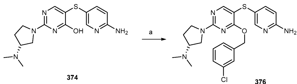
Scheme 60. Synthesis of 376.
