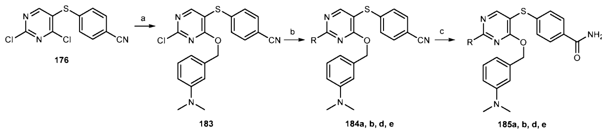
Scheme 27. Synthesis of 185a, b, d and e .
