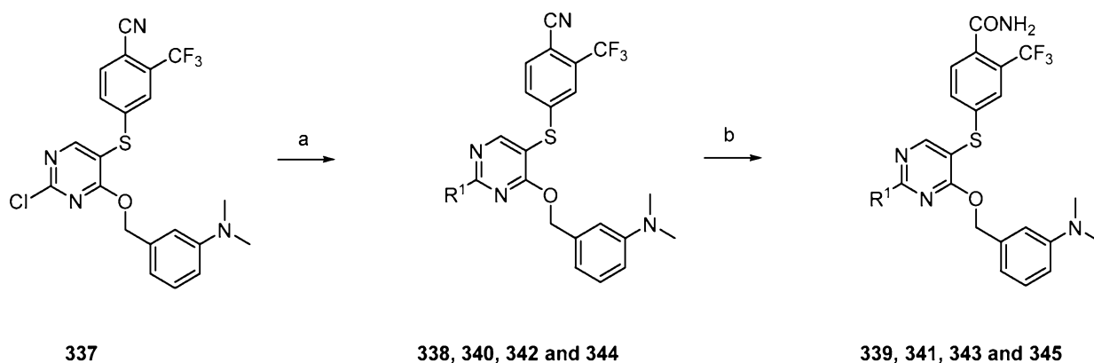
Scheme 52. Synthesis of 338-345.
