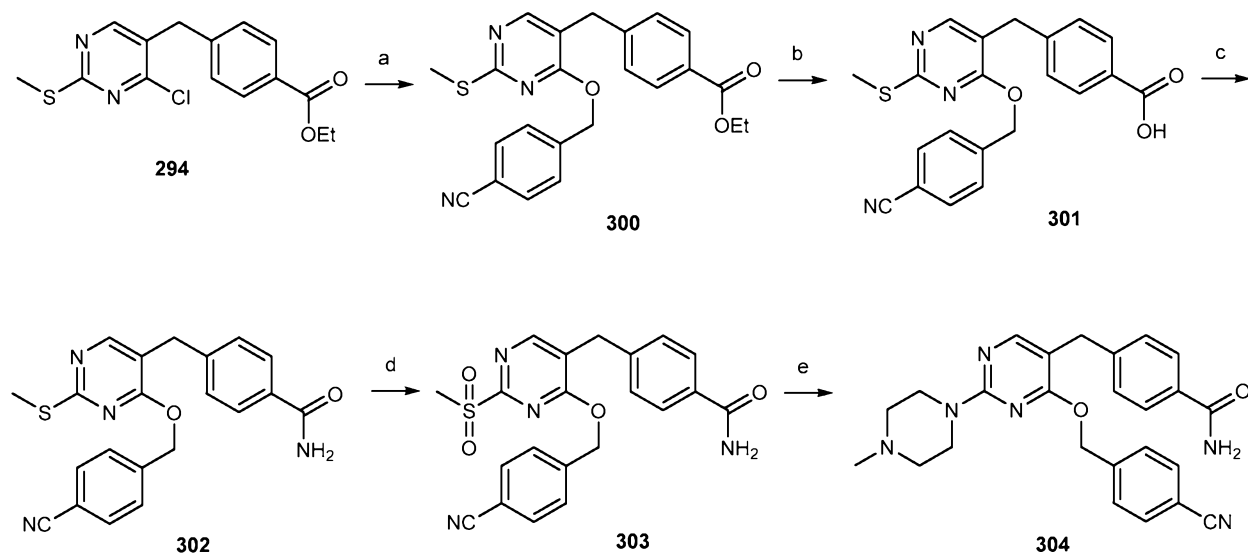
Scheme 46. Synthesis of 304 .
