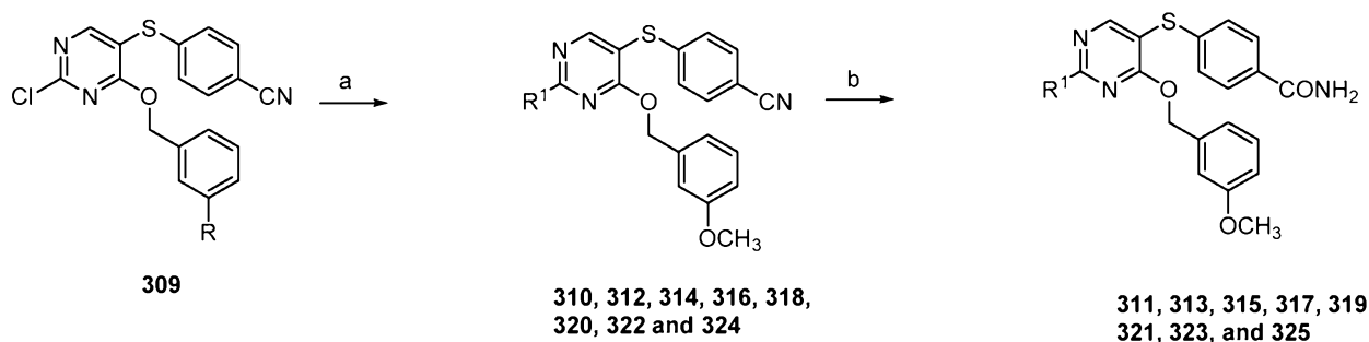
Scheme 48. Synthesis of 310-325
