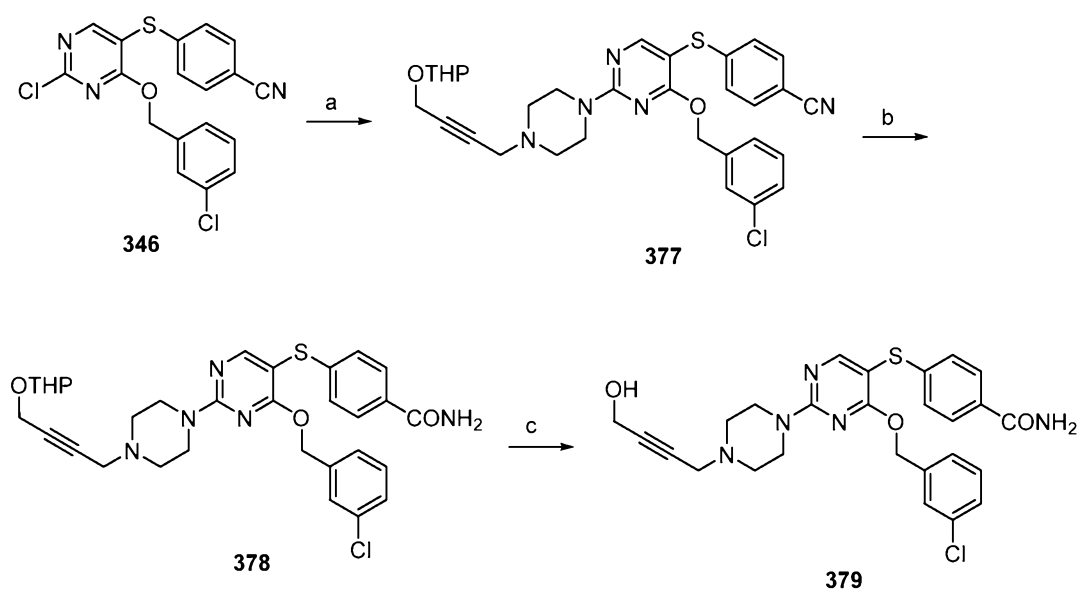
Scheme 61. Synthesis of 377-379.
