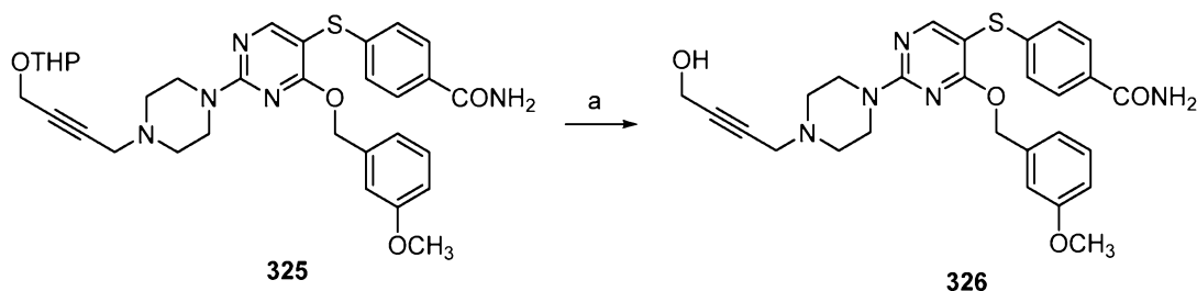
Scheme 49. Synthesis of 326.
