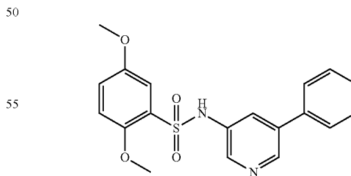
Example III-25: N-(5-Phenyl-pyridin-3-yl)-2,5-Dimethoxy-benzenesulfonamide
