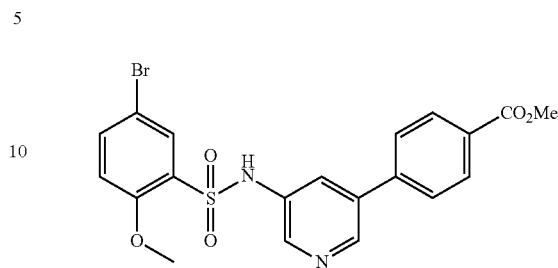
Example III-29: 4-[5-(5-Bromo-2-methoxy-benzenesulfonylamino)-pyridin-3-yl]-benzoic Acid Methyl Ester
