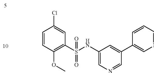
Example III-63: N-([3,3'-Bipyridin]-5-yl)-5-chloro-2-methoxybenzenesulfonamide
