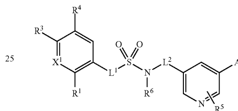
(Formula Ib)
