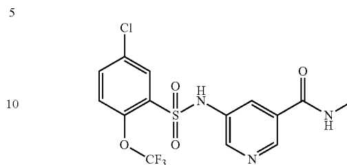
Example XII-6: 5-(5-Chloro-2-(trifluoromethoxy)phenylsulfonamido)-N-methylnicotinamide
