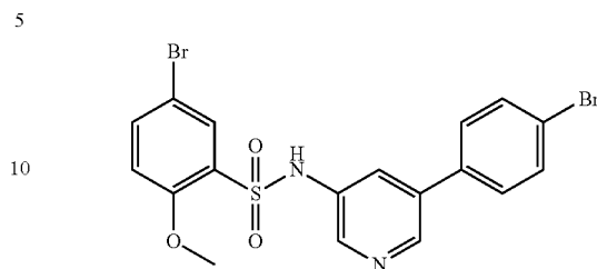
Example III-23: 5-Bromo-N-[5-(4-bromo-phenyl)-pyridin-3-yl]-2-methoxy-benzenesulfonamide
