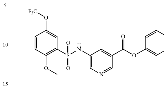
Example XII-18: Phenyl 5-(2-methoxy-5-(trifluoromethoxy)phenylsulfonamido)nicotinate
