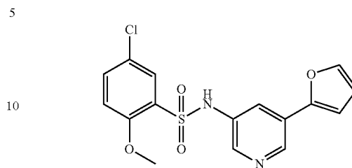
Example III-69: 5-Chloro-N-(5-(furan-2-yl)pyridin-3-yl)-2-methoxybenzenesulfonamide
