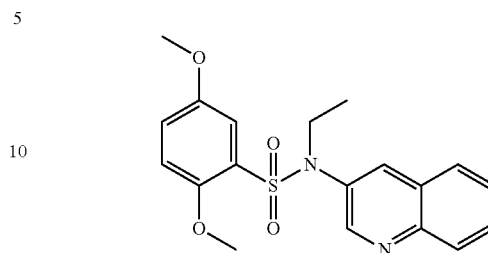
Example VII-13: 2,5-Dimethoxy-N-ethyl-N-(quinolin-3-yl)benzenesulfonamide
