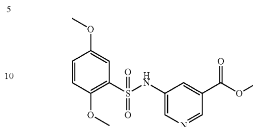
Example IV-11: Methyl 5-(2,5-dimethoxyphenylsulfonamido)nicotinate
