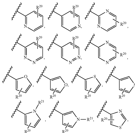
(Formula IVd)
