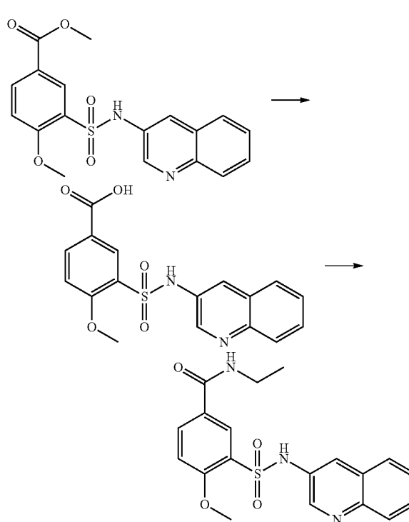
Example II-16: N-Ethyl-4-methoxy-3-(quinolin-3-ylsulfamoyl)-benzamide
