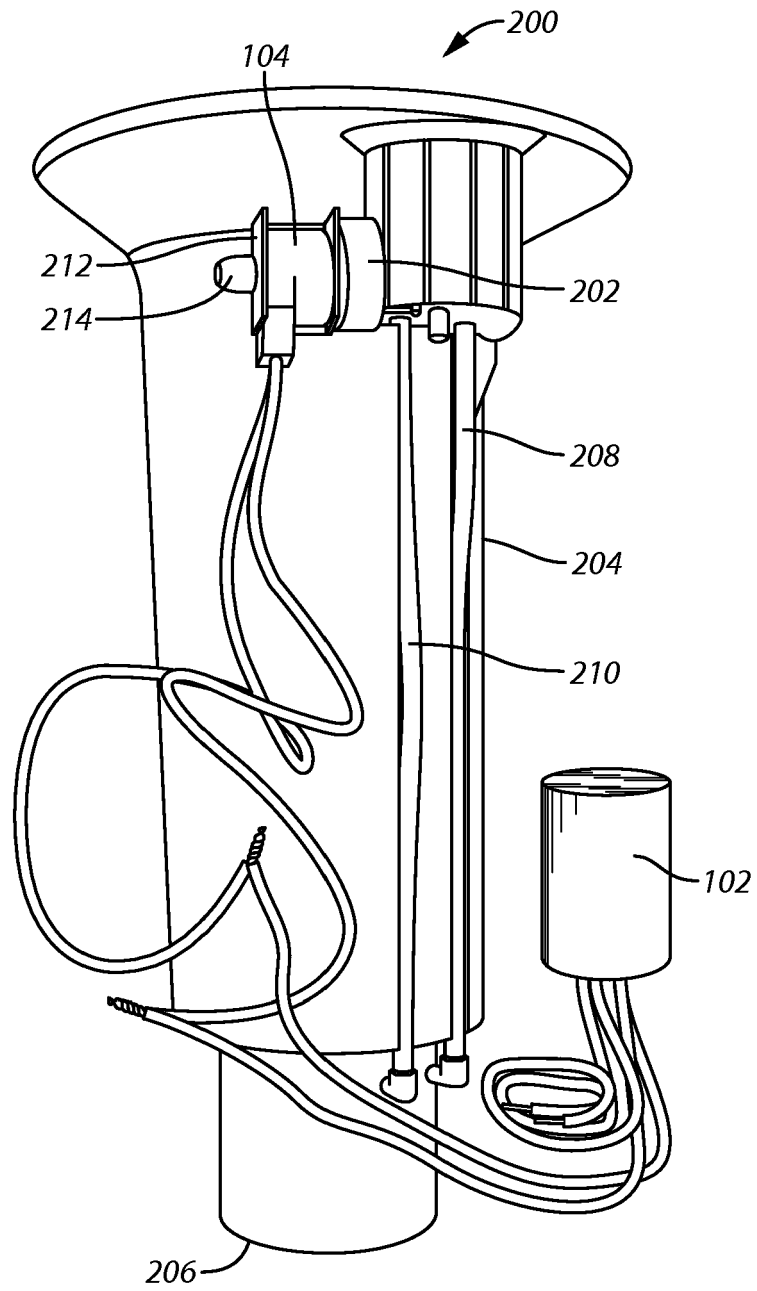
FIG. 2 (Prior Art)
