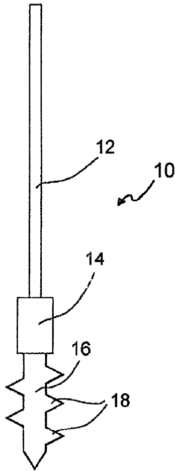
Fig. 1 (PRIOR ART)
