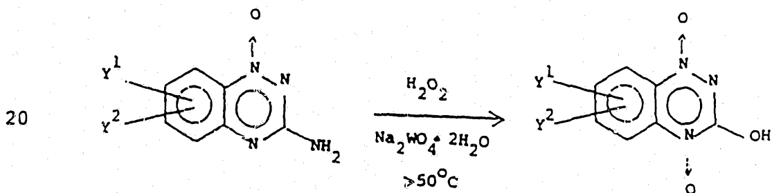
Scheme III
