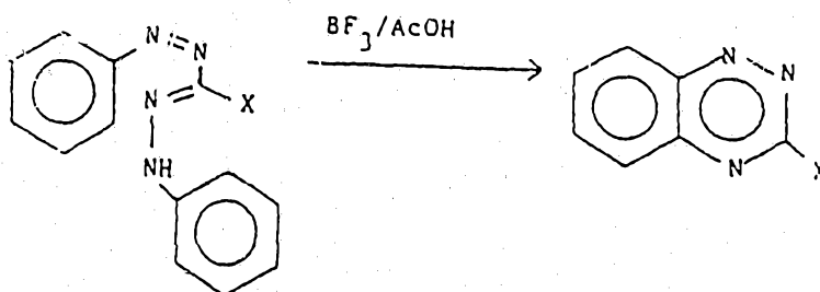
Scheme I
