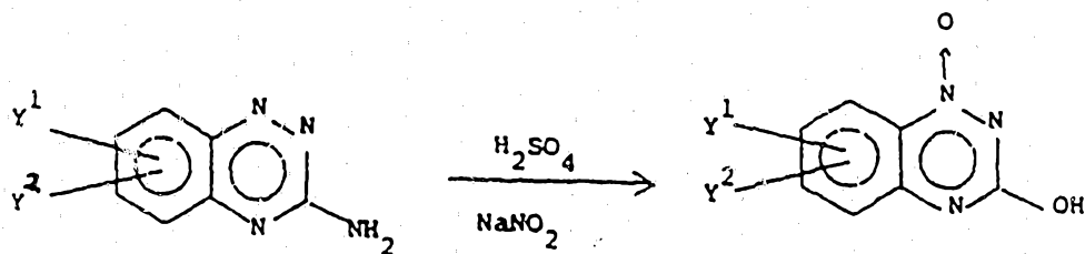
Scheme III
