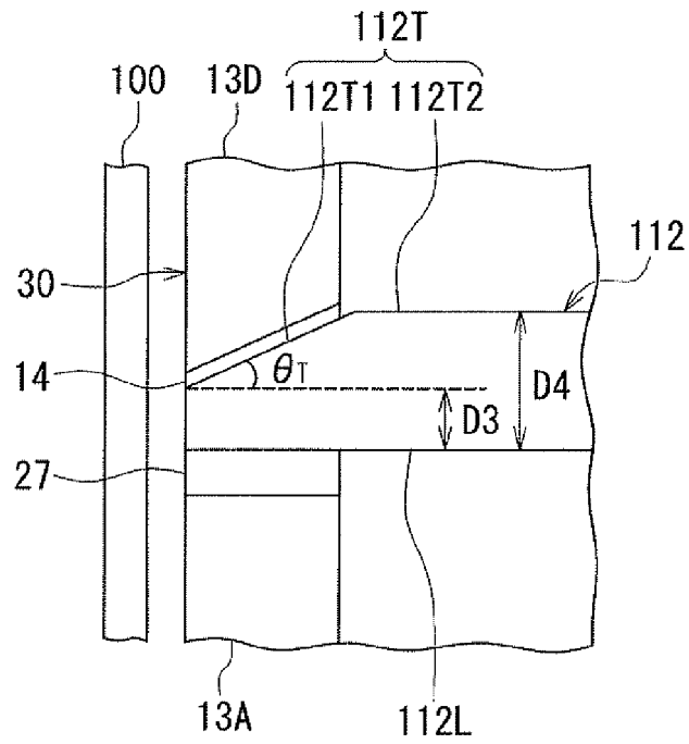
FIG. 15 RELATED ART
