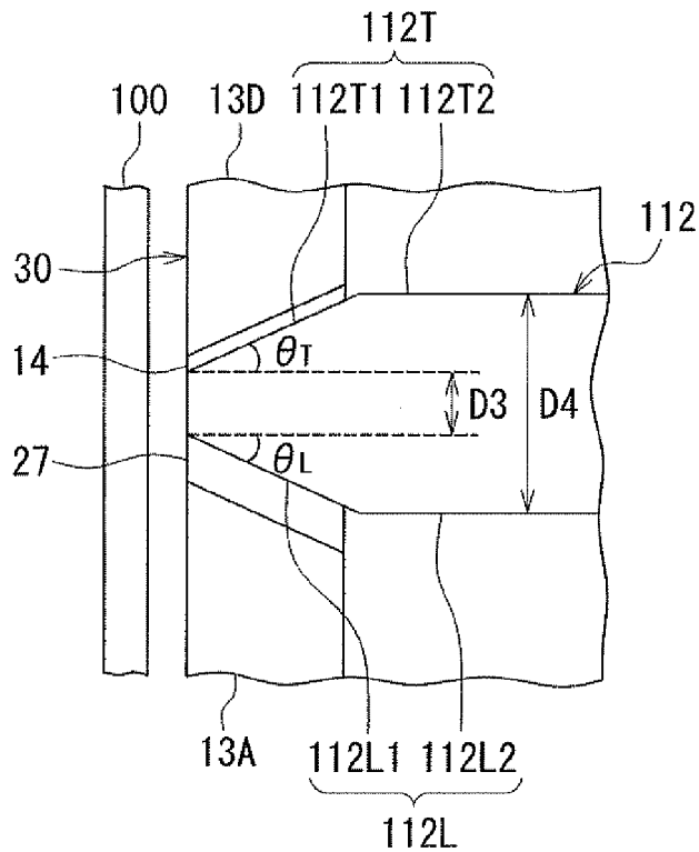
FIG. 16 RELATED ART
