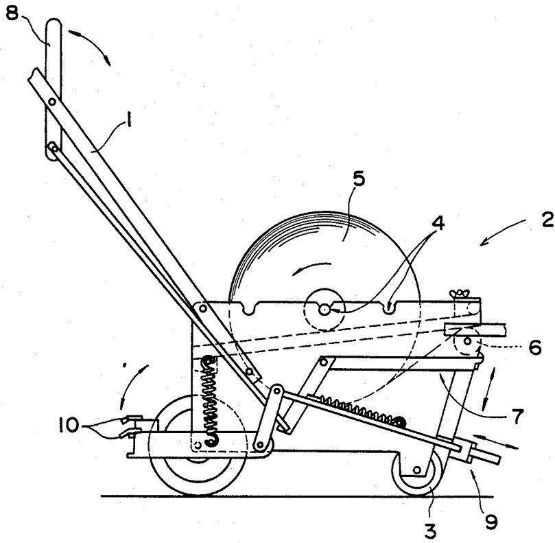
FIG. 10 PRIOR ART
