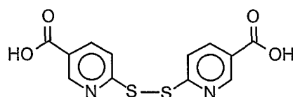
Dithionicotinic acid
