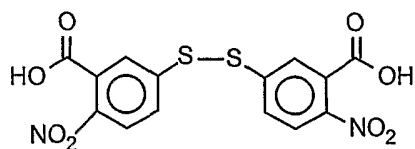
Ellman's reagent
