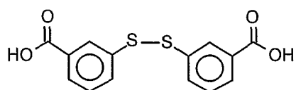
dithiosalicylic acid
