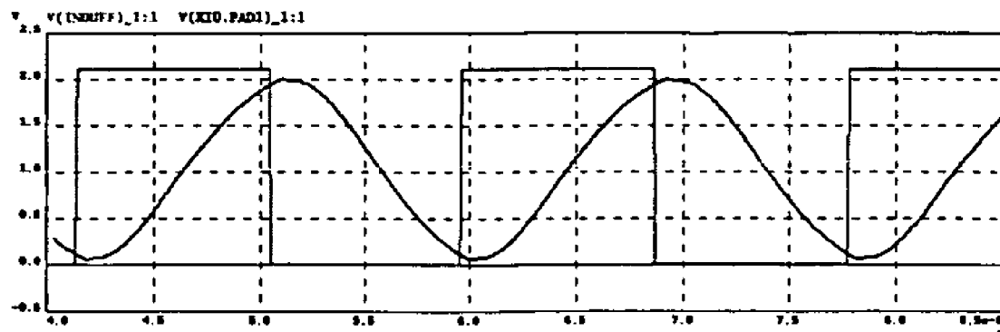
Input & output to the output driver
