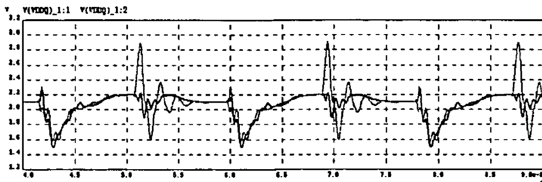
Supply Noise with/without additional circuit
