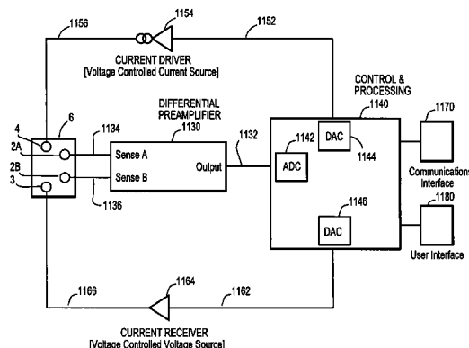
Galvanodynamic Test System
