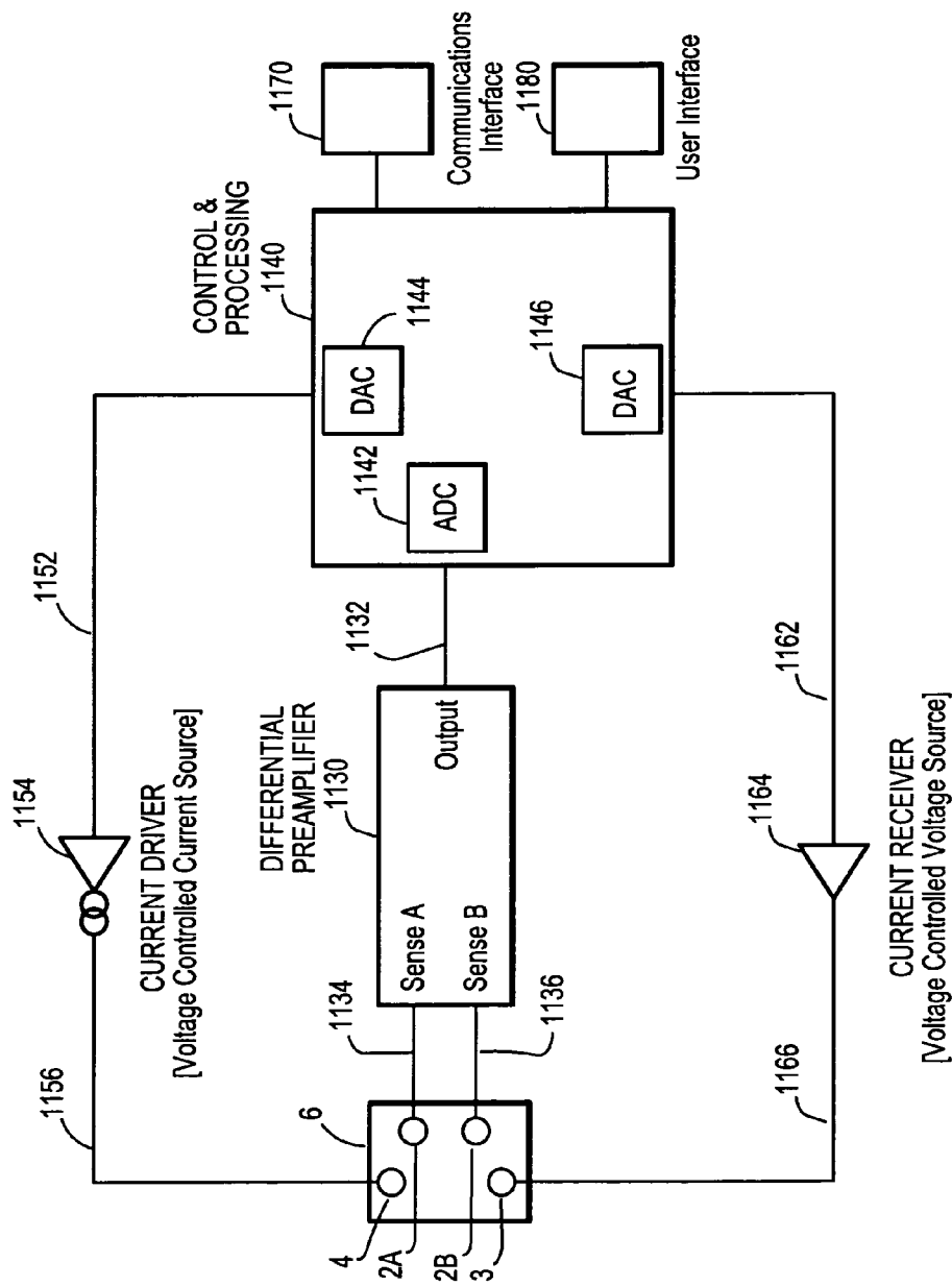
FIG. 11 Galvanodynamic Test System
