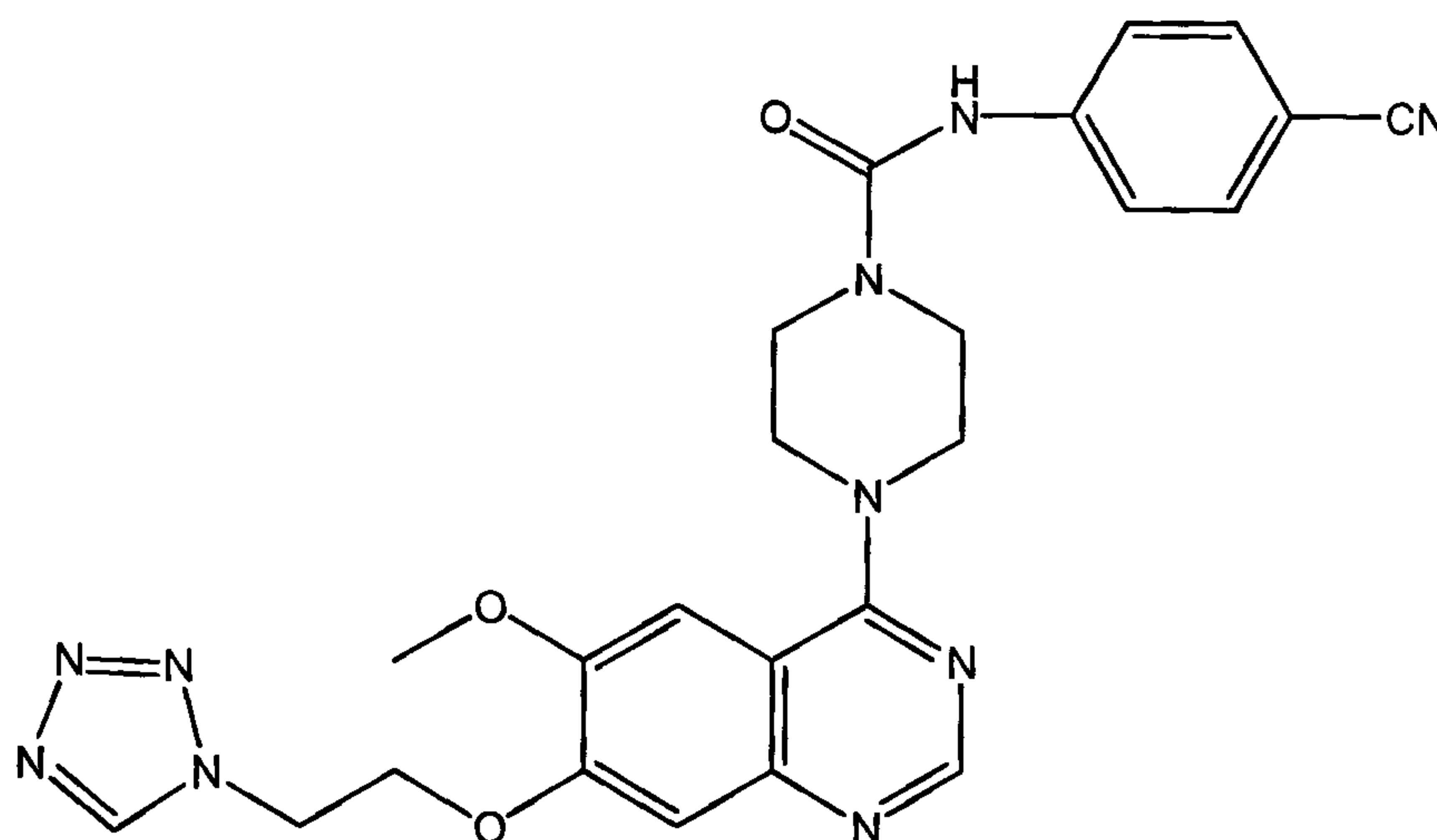
N-(4-cyanophenyl){4-[6-methoxy-7-(2-(1,2,3,4-tetraazolyl)ethoxy)quinazolin-4-yl]piperazinyl}carboxamide
