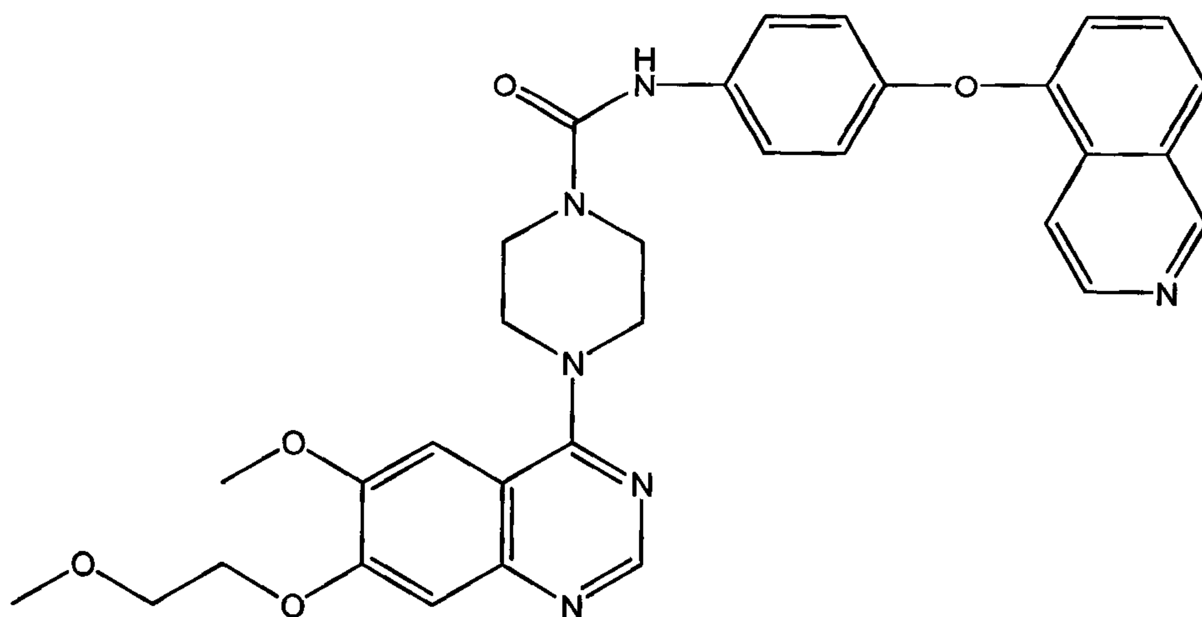
N-(4-(5-isoquinolyloxy)phenyl){4-[6-methoxy-7-(2-methoxyethoxy)quinazolin-4-yl]piperazinyl}carboxamide
