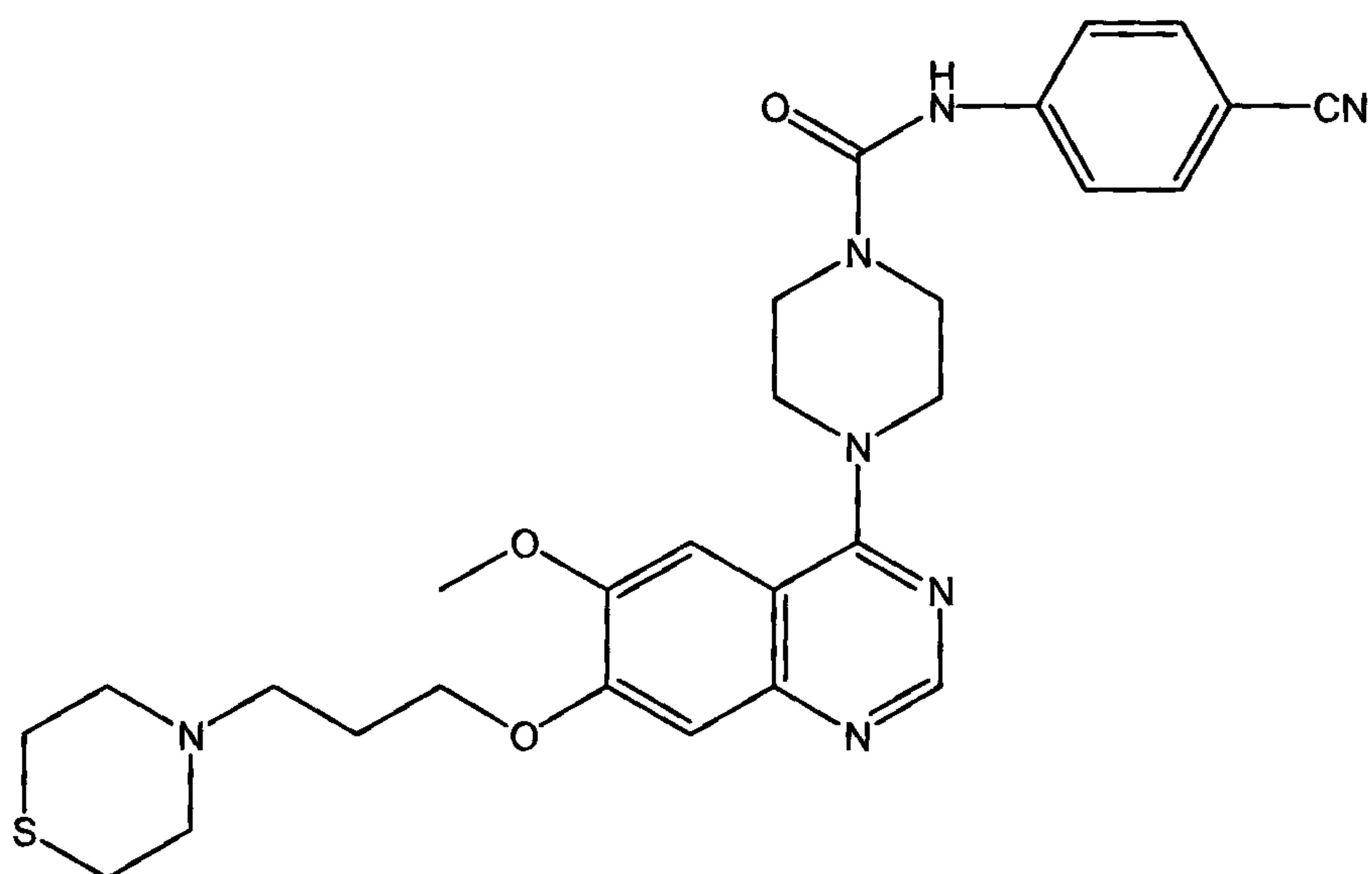
(4-{7-[3-(1,1-dioxo(1,4-thiazaperhydroin-4-yl))propoxy]-6-methoxyquinazolin-4-yl}piperazinyl)-N-(4-cyanophenyl)carboxamide
