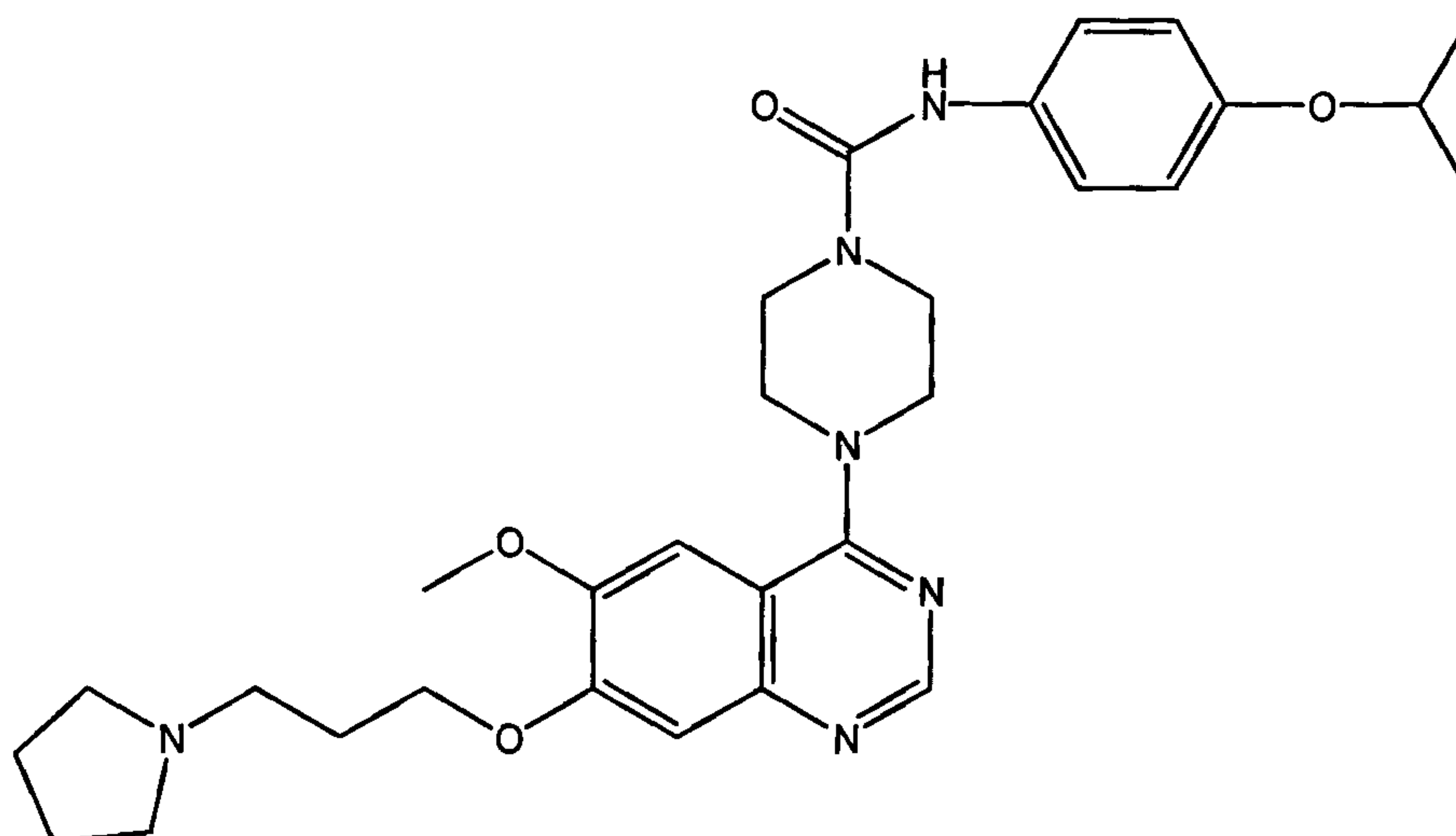
N-(4-cyanophenyl){4-[6-methoxy-7-(2-(1,2,3,4-tetraazol-2-yl)ethoxy)quinazolin-4-yl]piperazinyl}carboxamide
