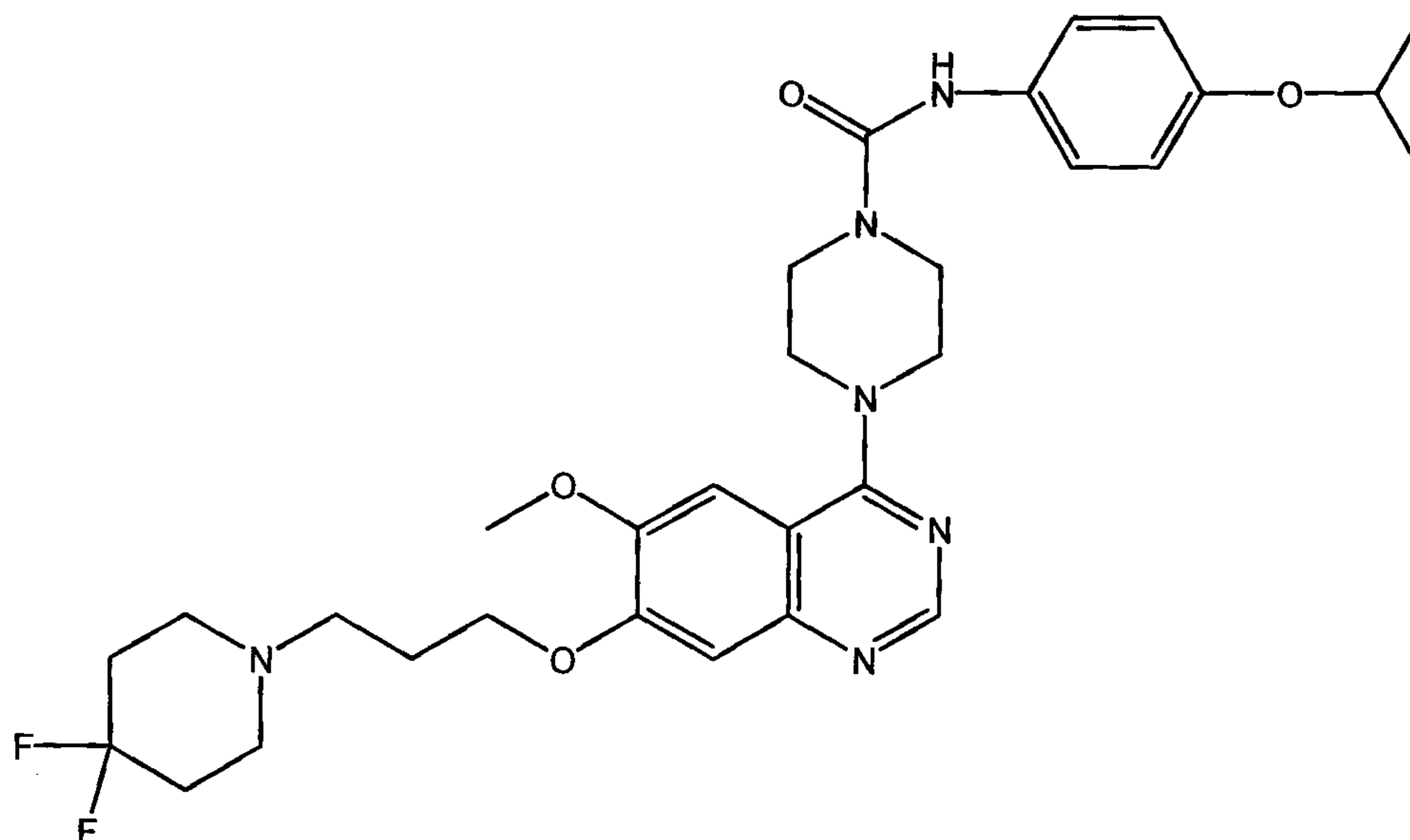
{4[6-methoxy-7-(3-piperazinylpropoxy)quinazolin-4-yl]piperazinyl}-N-[4-(methylethoxy)phenyl]carboxamide
