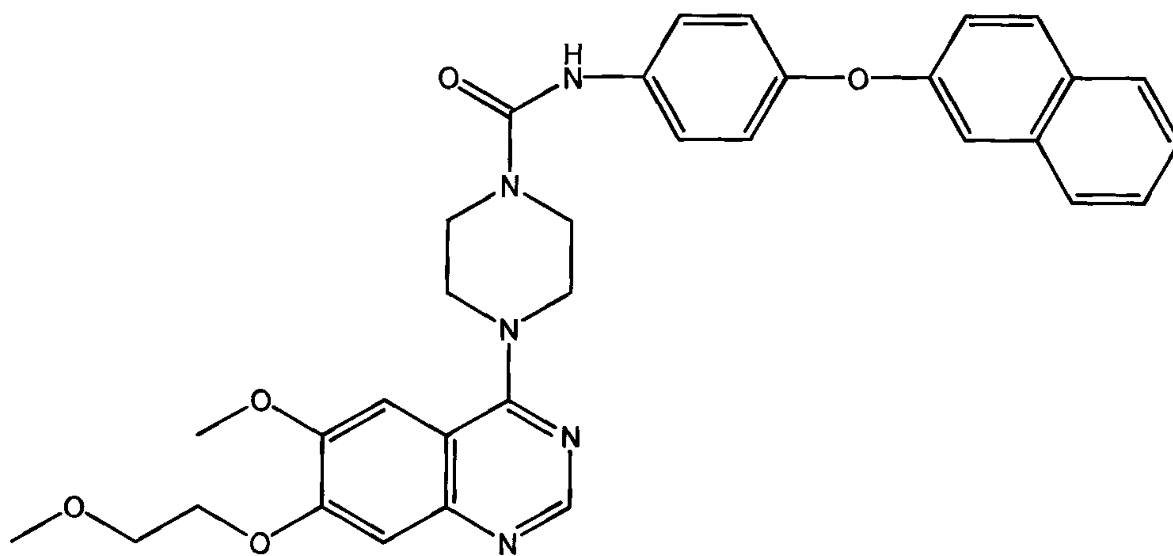
N-(4-(5-isoquinolyloxy)phenyl){4-[6-methoxy-7-(2-methoxyethoxy)quinazolin-4-yl]piperazinyl}carboxamide
