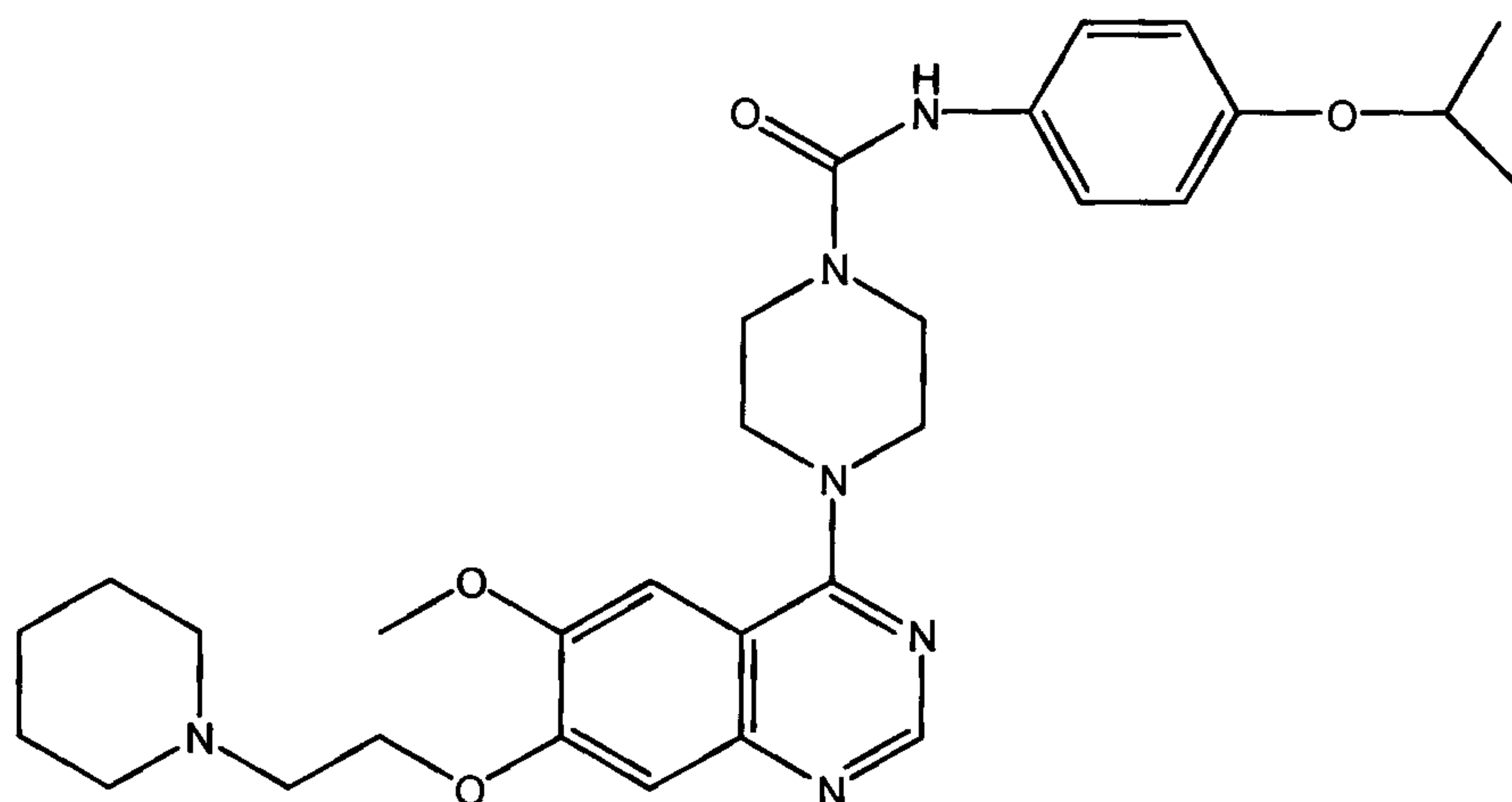
N-(4-cyanophenyl){4-[6-methoxy-7-(2-piperidylethoxy)quinazolin-4-yl]piperazinyl}carboxamide
