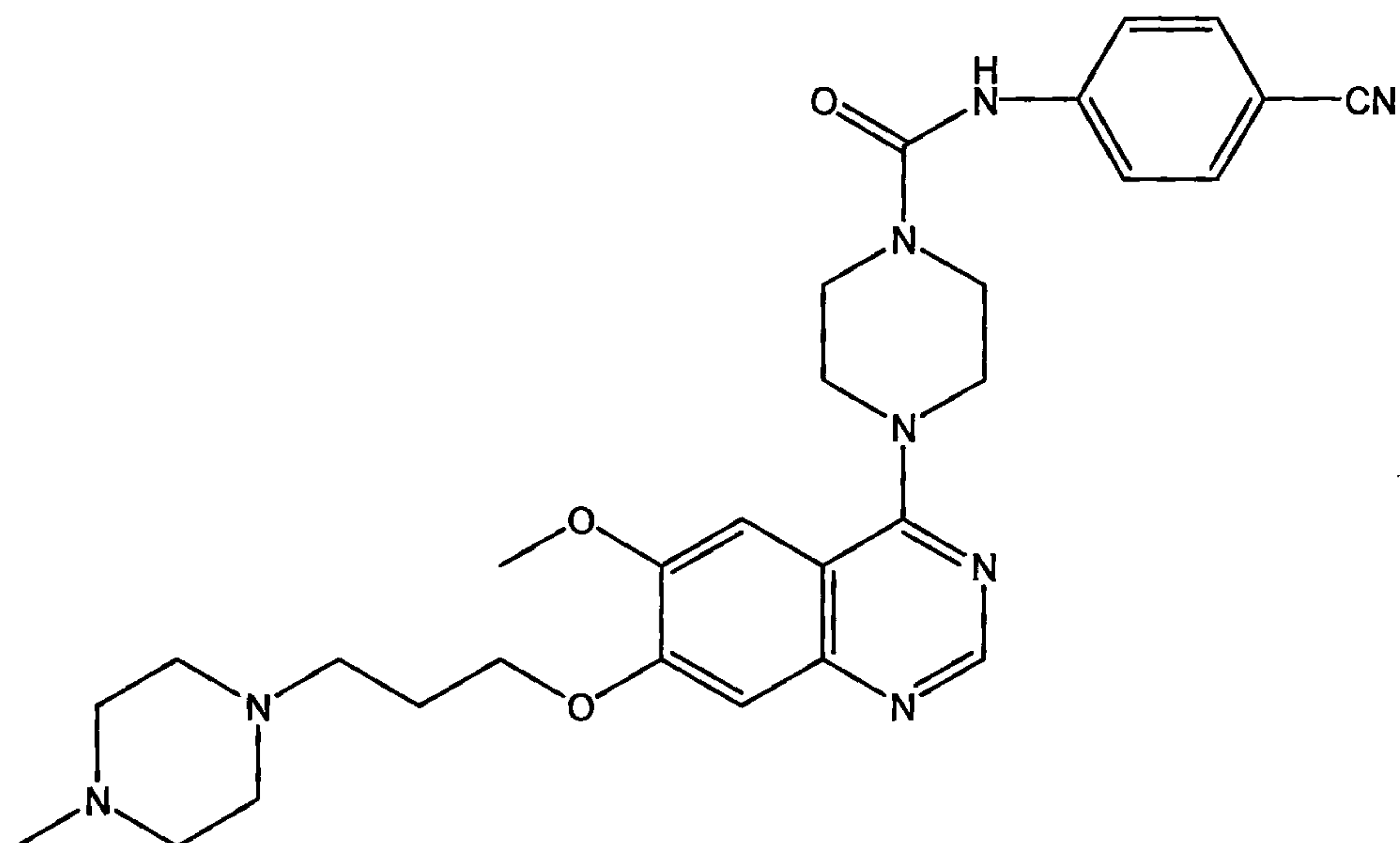
N-(4-cyanophenyl){4-[6-methoxy-7-(3-(1,4-thiazaperhydroin-4-yl)propoxy)quinazolin-4-yl]piperazinyl}carboxamide
