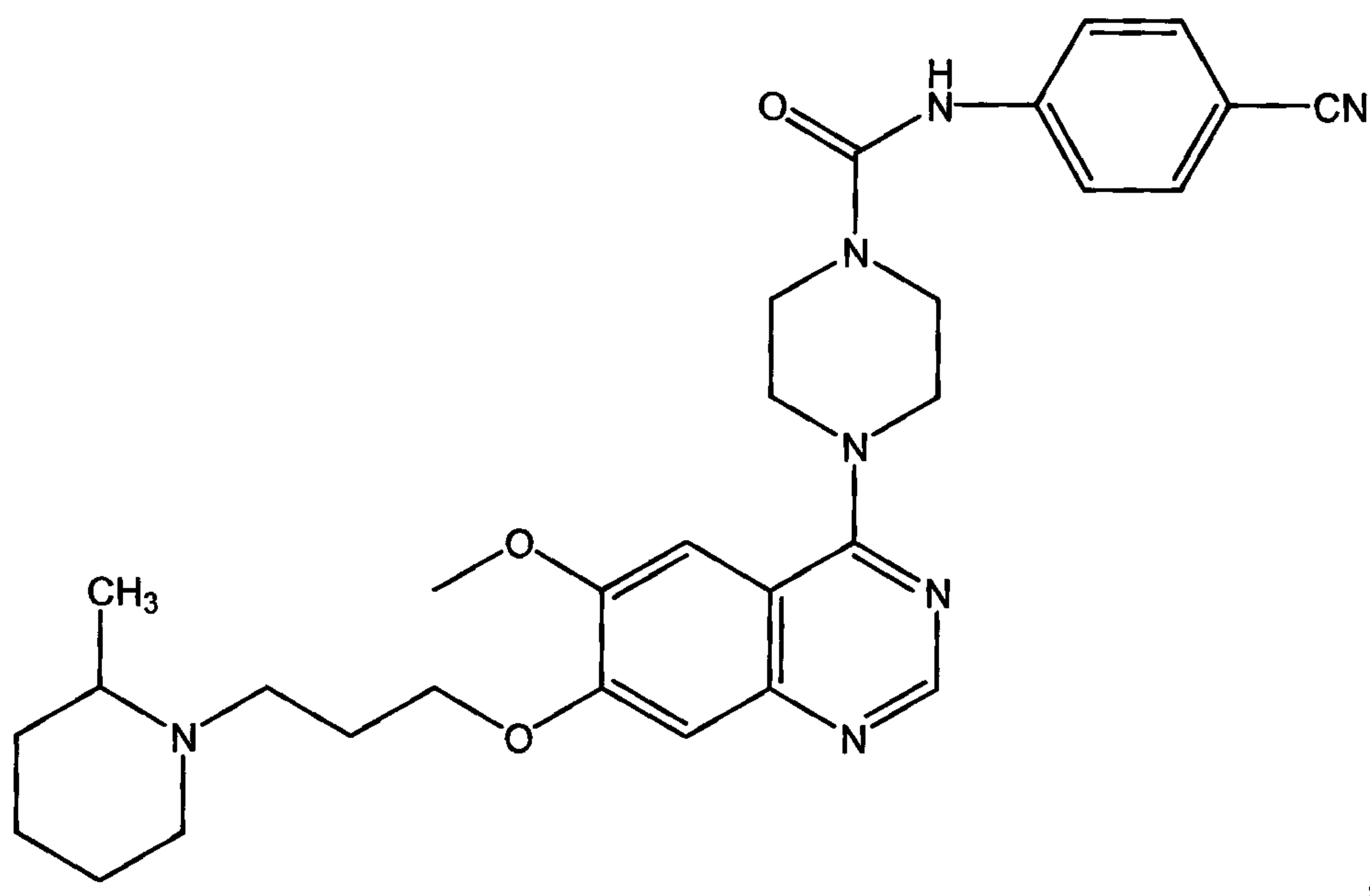
N-(4-cyanophenyl)(4-{6-methoxy-7-[3-(4-methylpiperidyl)propoxy]quinazolin-4-yl}piperazinyl)carboxamide
