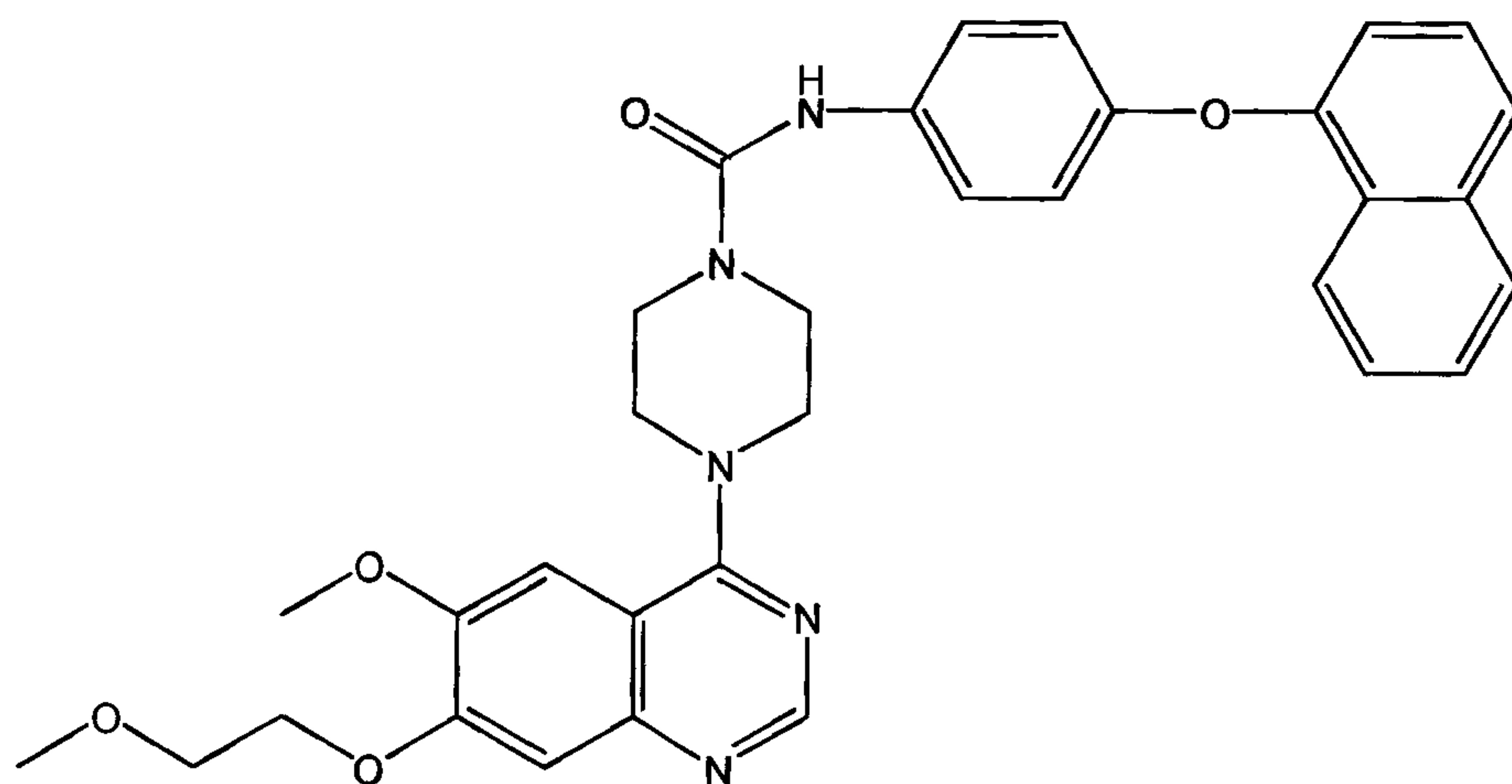
{4-[6-methoxy-7-(2-methoxyethoxy)quinazolin-4-yl]piperazinyl}-N-(4-(2-naphthyloxy)phenyl)carboxamide
