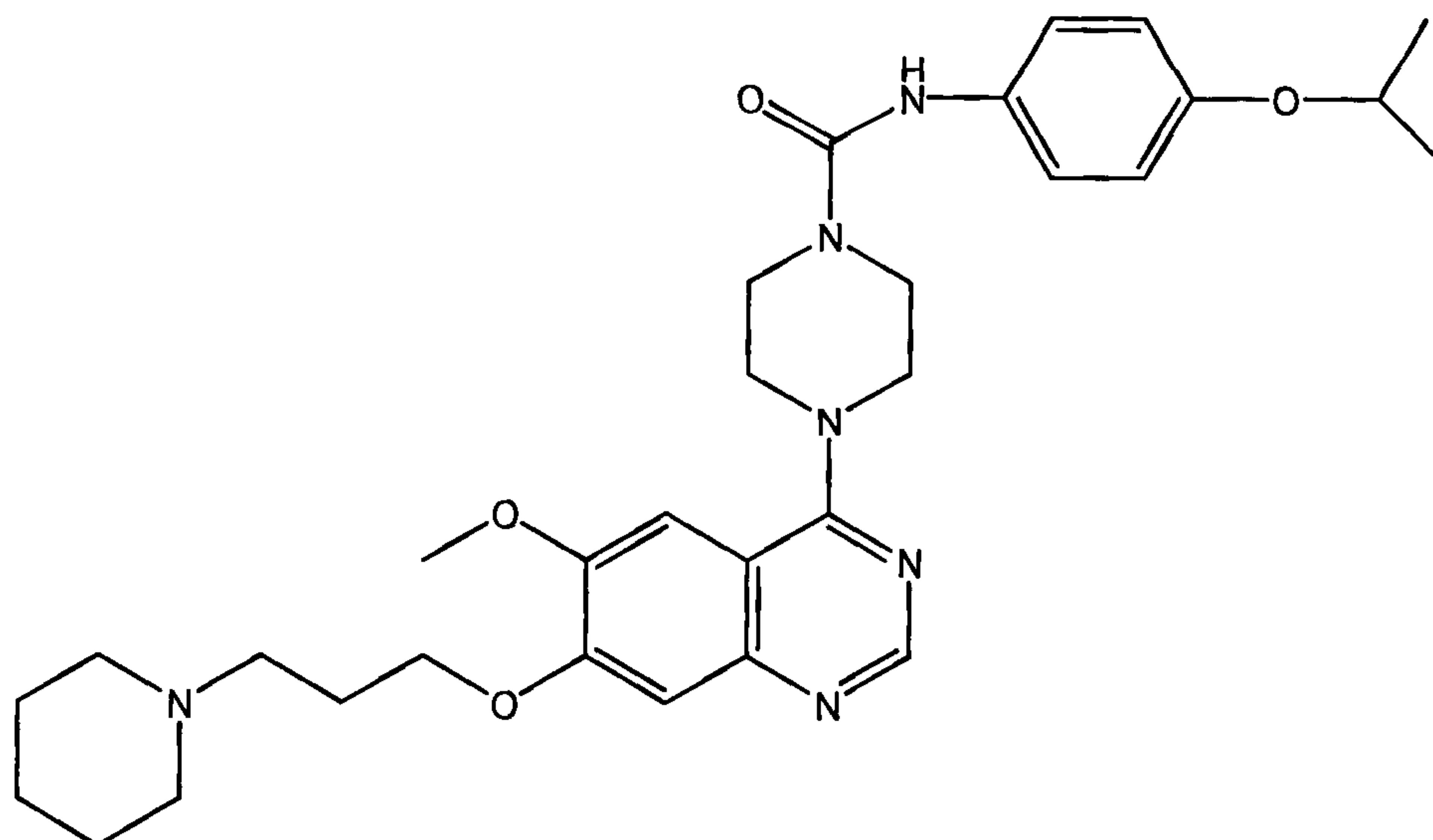
{4-[6-methoxy-7-(3-piperidylpropoxy)quinazolin-4-yl]piperazinyl}-N-[4-(methylethoxy)phenyl]carboxamide
