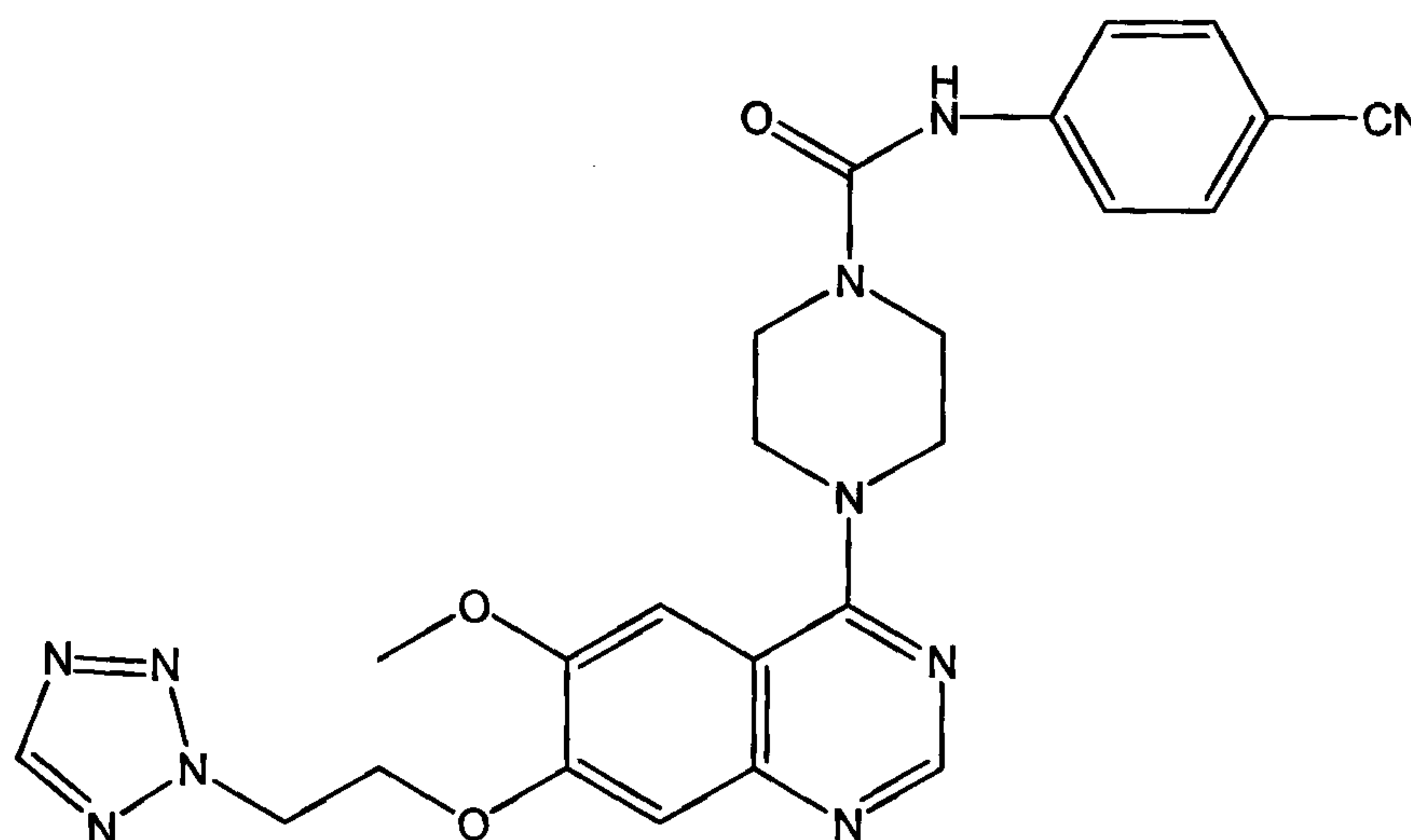
N-(4-cyanophenyl){4-[6-methoxy-7-(2-(1,2,3,4-tetraazolyl)ethoxy)quinazolin-4-yl]piperazinyl}carboxamide
