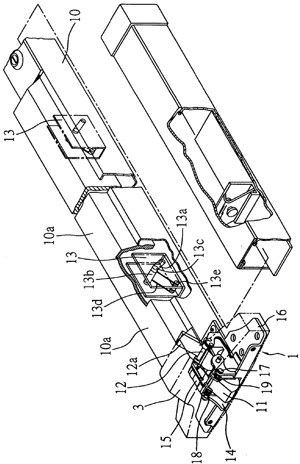
FIG. 2 (PRIOR ART)
