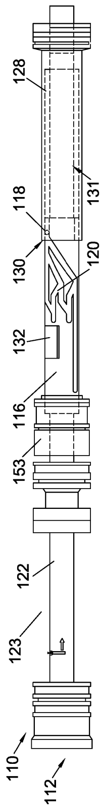
Fig. 6 Tool overview. Housing and the return spring omitted for clarity
