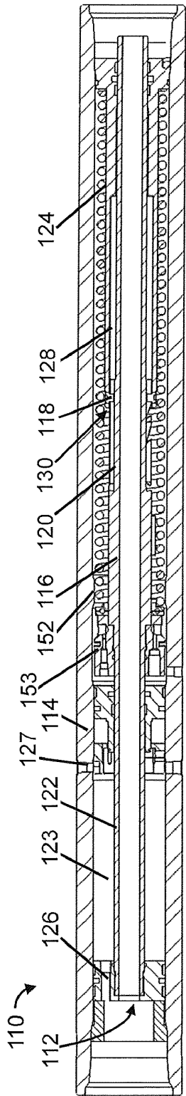
Fig.3 NO FLOW - TOOL CLOSED
