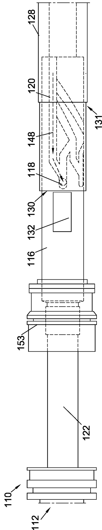
Fig. 8 Position 2. Flow on. The Driving Piston over-rides the Return spring, moving the Mandrel downwards. The J Slot and J Pin rotates the Mandrel until it no-go's.
