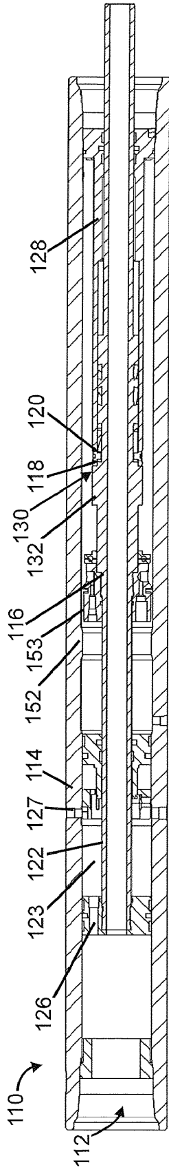
Fig.4 FLOW ON - SHORT STROKE - NOT ACTUATED
