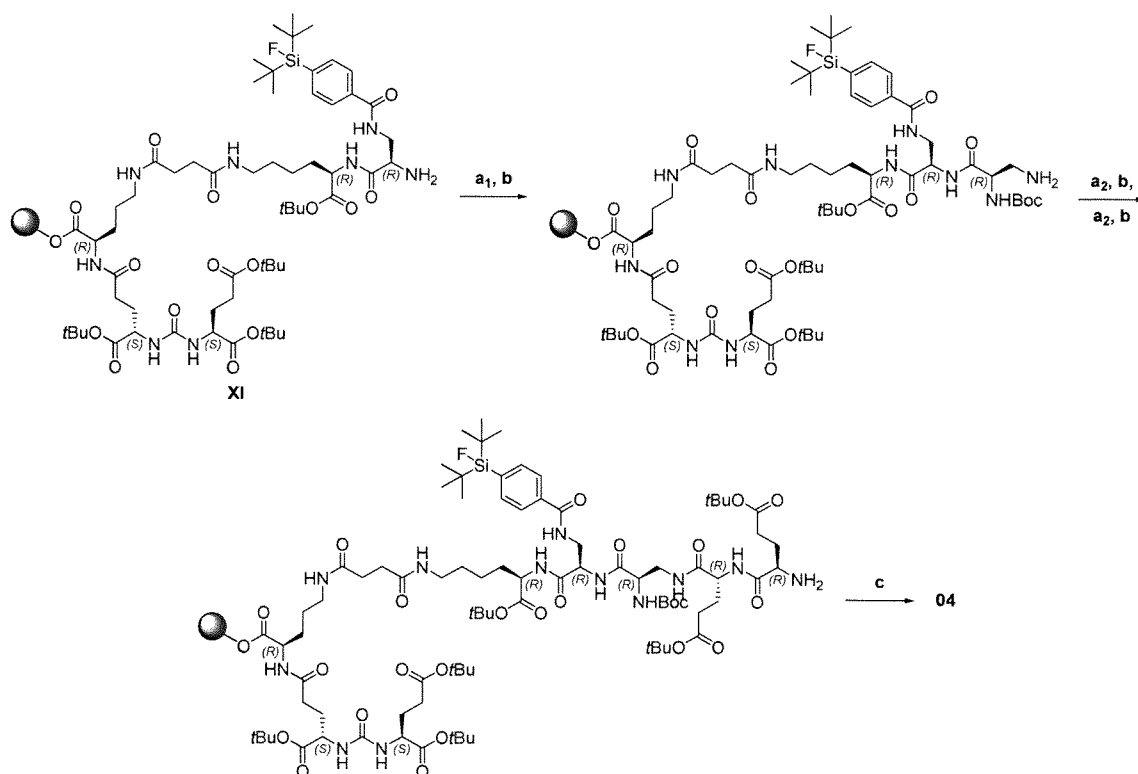
Scheme 14. Synthesis of SiFA-PSMA ligand 04 : a_1 ) Boc-D-Dap(Fmoc)-OH, HOAt, TBTU, sym -collidine, (DMF); a_2 ) Fmoc-D-Glu(OtBu)-OH, HOAt, TBTU, sym -collidine, (DMF); b ) 20% Pip in DMF; c ) 95% TFA/2.5% TIPS/2.5% water.
