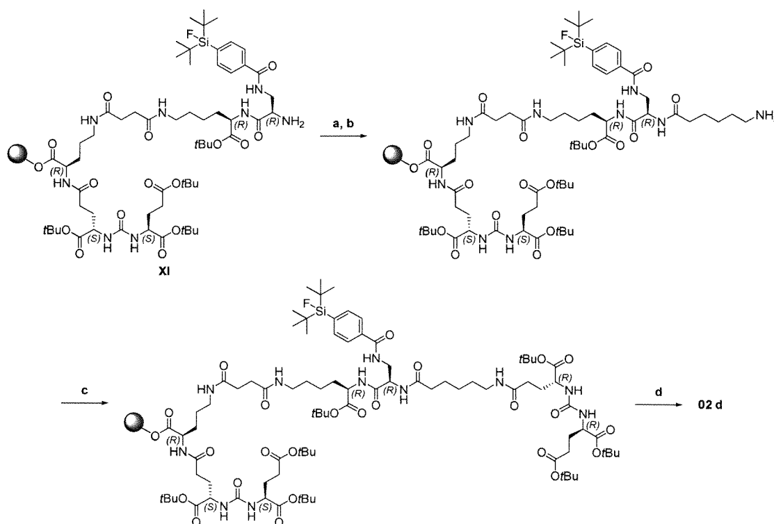
Scheme 11. Synthesis of SiFA-PSMA ligand 02 d : a) Fmoc-Ahx-OH, HOAt, TBTU, sym -collidine, (DMF); b) 20% Pip in DMF; c) t BuO-D-Glu(OTBu)-u-D-Glu-OTBu ( XV ), HOAt, TBTU, sym -collidine, (DMF); d) 95% TFA/2.5% TIPS/2.5% water.
