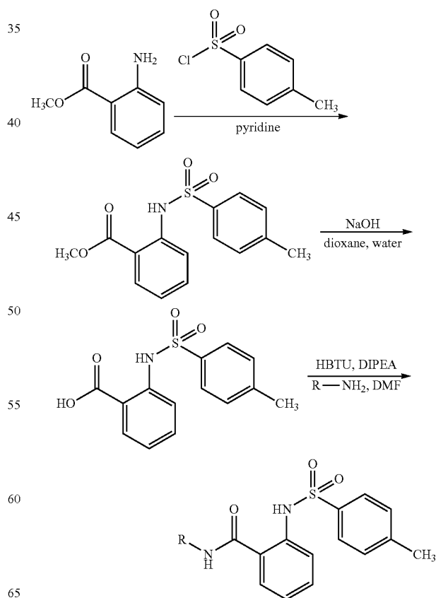
Scheme 2. Representative synthesis of amide analogues via carboxylate
