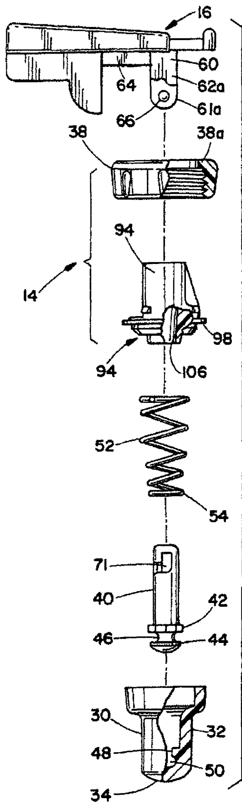
FIG. 4 (PRIOR ART)
