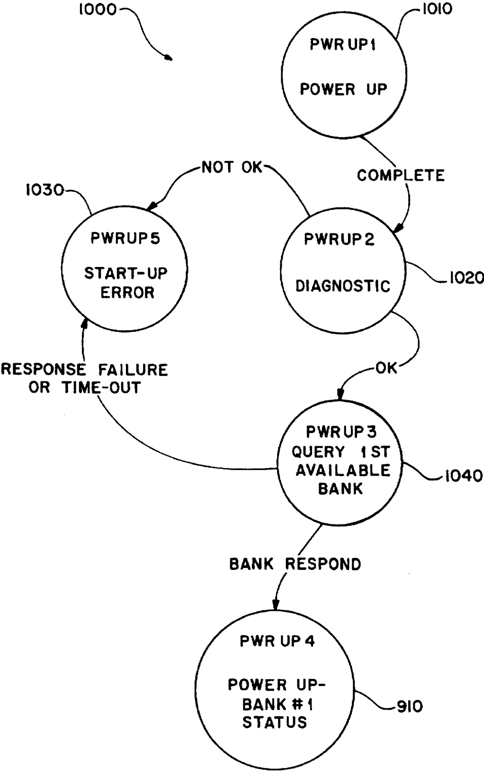
FIGURE 10 POWER UP
