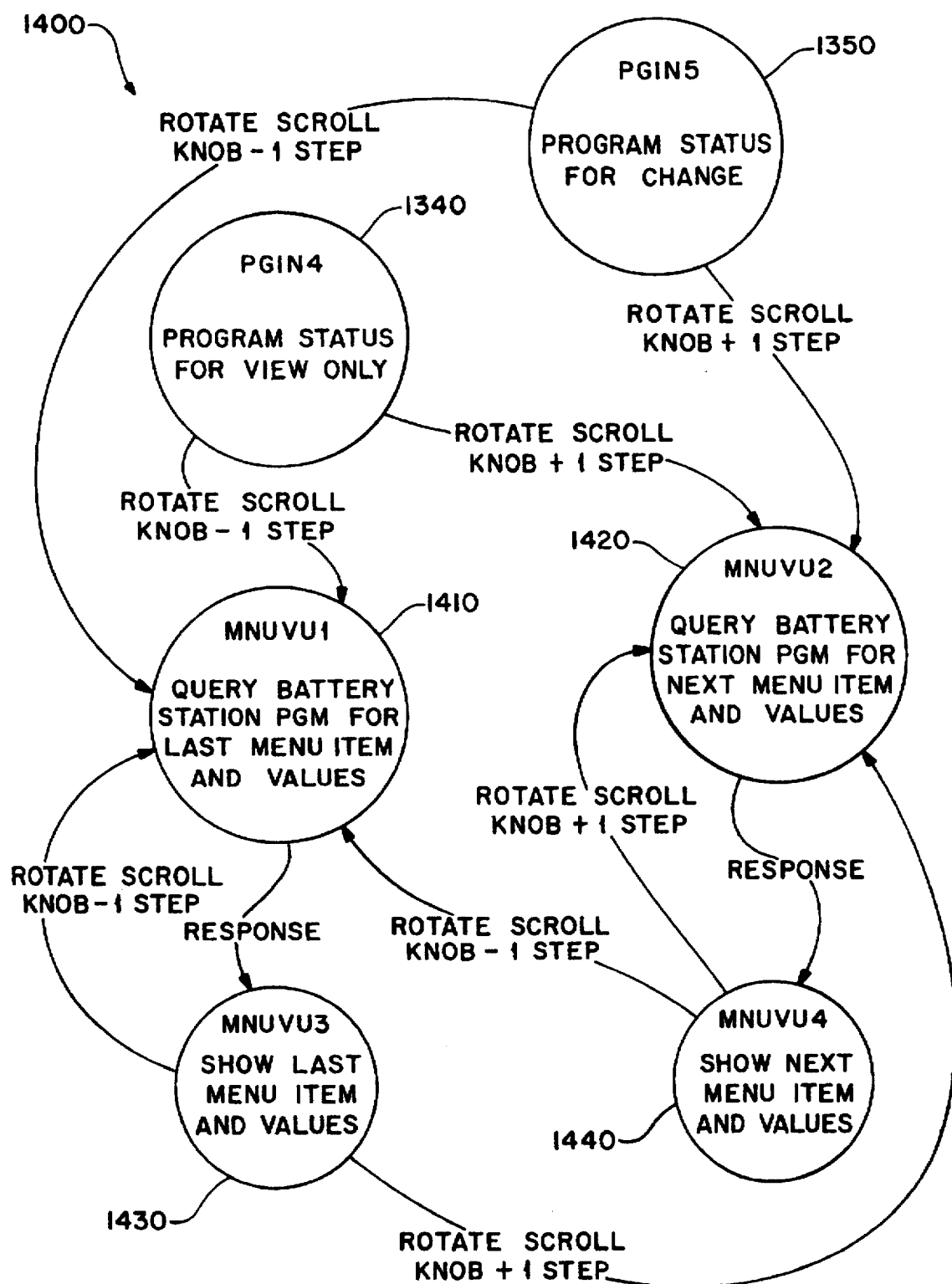
FIGURE 14 PROGRAM MENU
