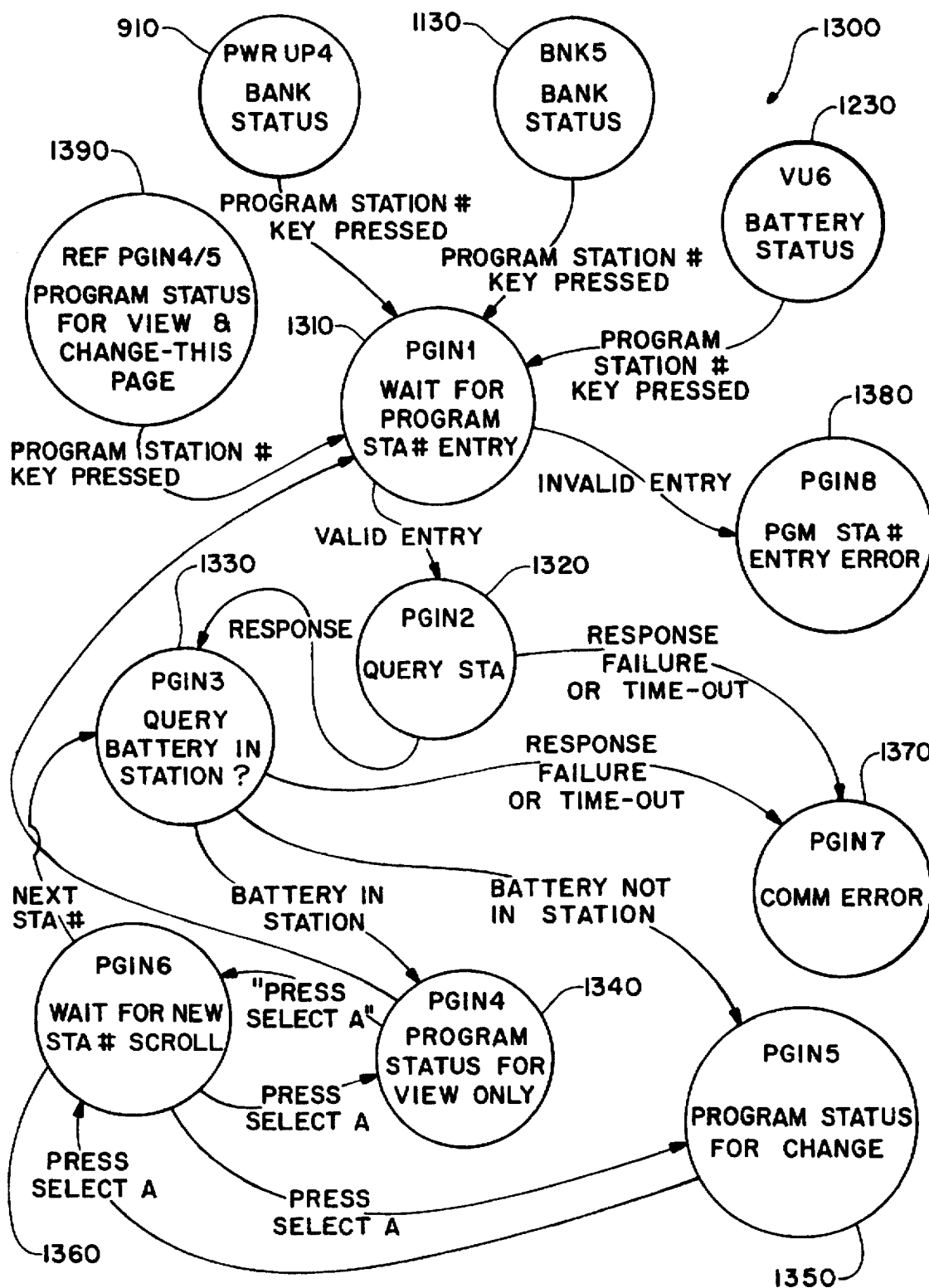
FIGURE 13 PROGRAM INITIALIZE
