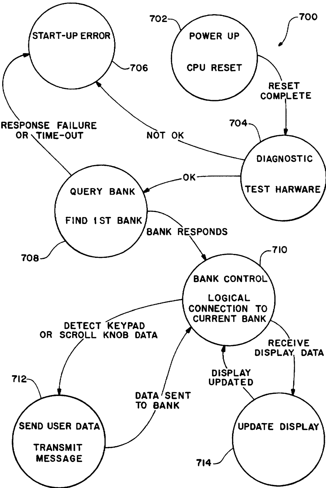
FIGURE 7 REMOTE CONTROL UNIT
