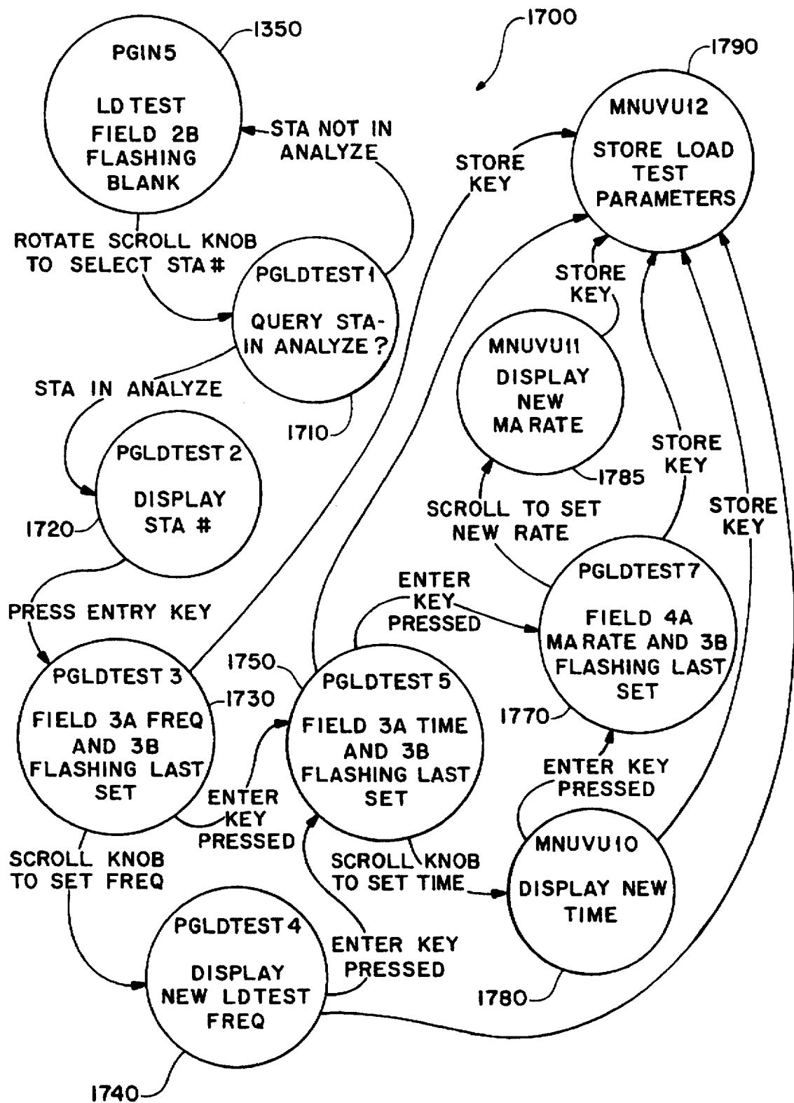
FIGURE 17 LOAD TEST
