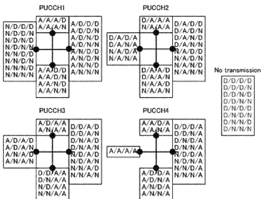
Figure 5 Mapping rules in case that four DL CCs are configured (Alternative 1-2)
