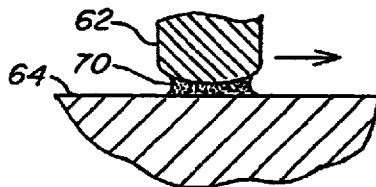
Fig. 6c (PRIOR ART)
