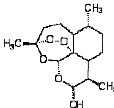
Dihydroartemisinin
