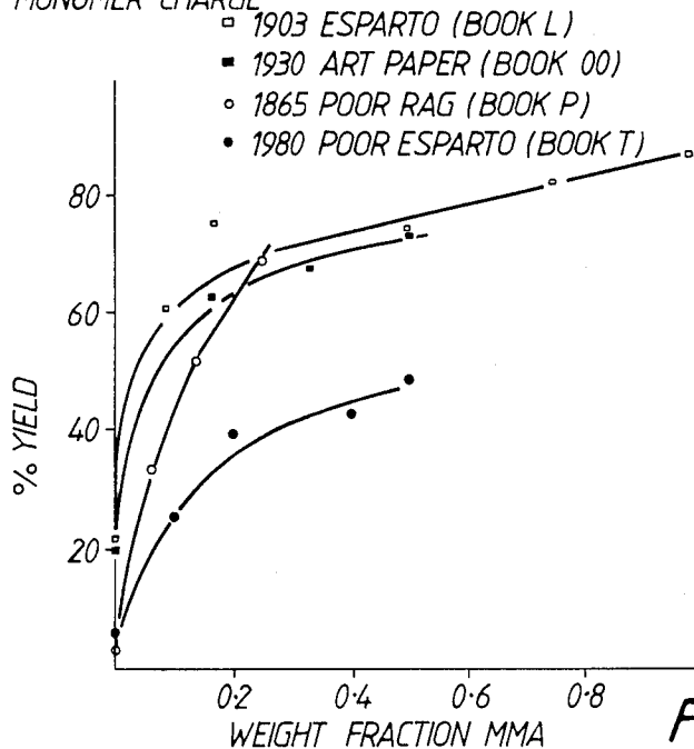
DEPENDENCE OF YIELD ON WEIGHT FRACTION METHYL METHACRYLATE IN MONOMER CHARGE
