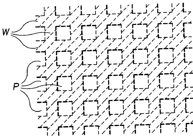
Fig. 7 (PRIOR ART)
