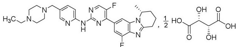
Formula II (compound II)
