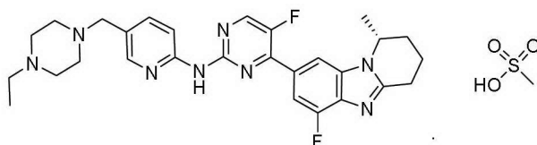
Formula III (compound III)
