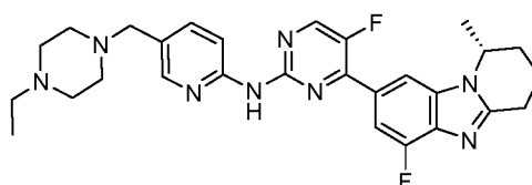
Formula I (compound I)
