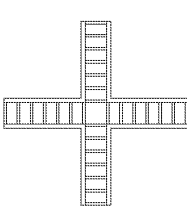
Holliday Structure
