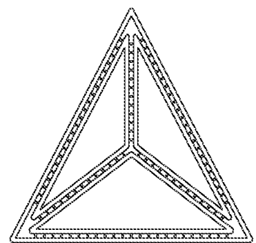
Tetrahedron
