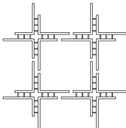
2-D Crystal
