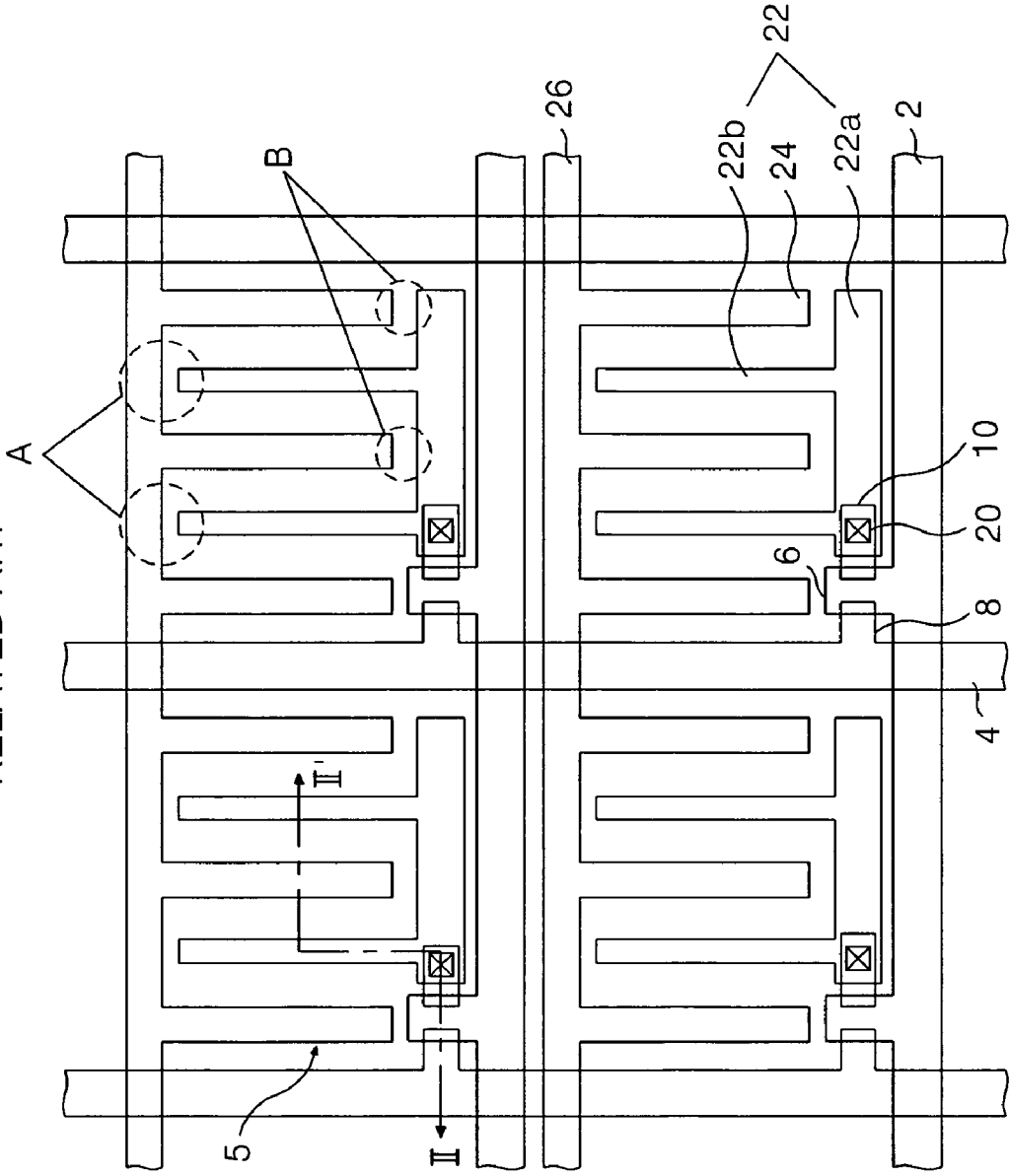
FIG. 1 RELATED ART
