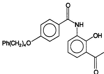
(IIIA)
