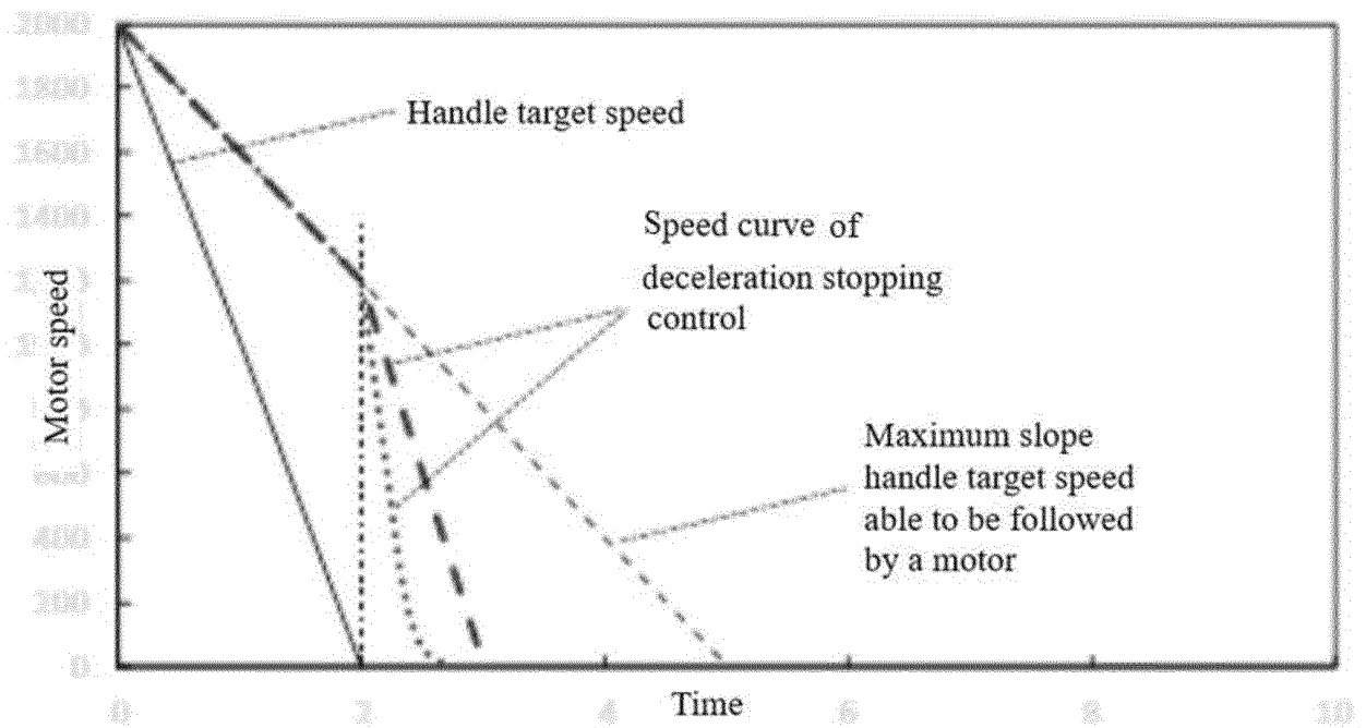
(b) Handle displacement changes rapidly
