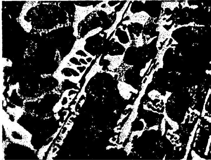
500:1 Etched with Nital White: Carbide of the Ledeburite Gray: Pearlite of the Ledeburite Black: Graphite
