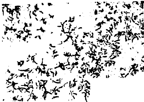
100:1 Unetched Graphite Formation
