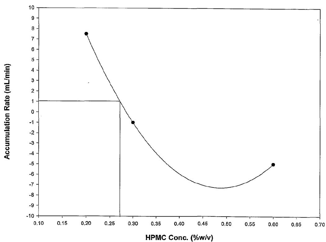
Figure 2. Irrigating solution accumulation at the default settings of Legacy 20000 and at maximum possible vacuum.
