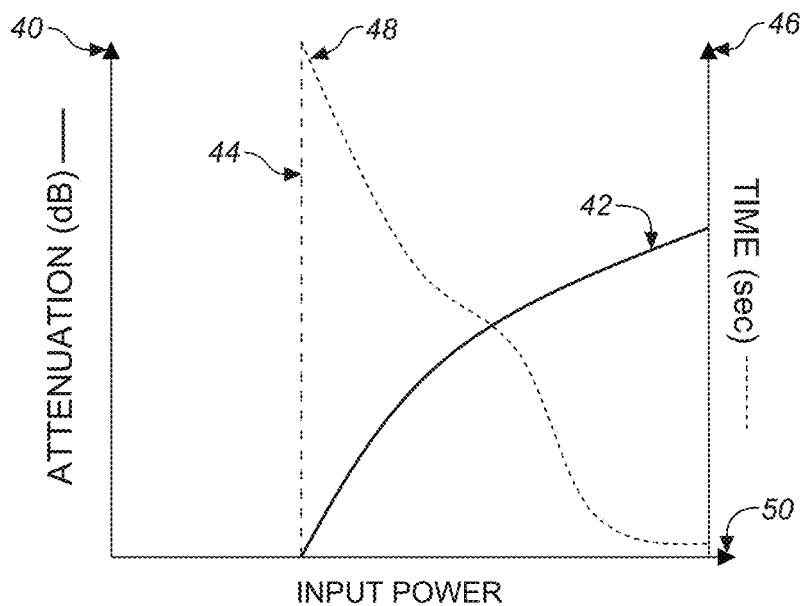
Typical Loudspeaker Power Handling Performance
