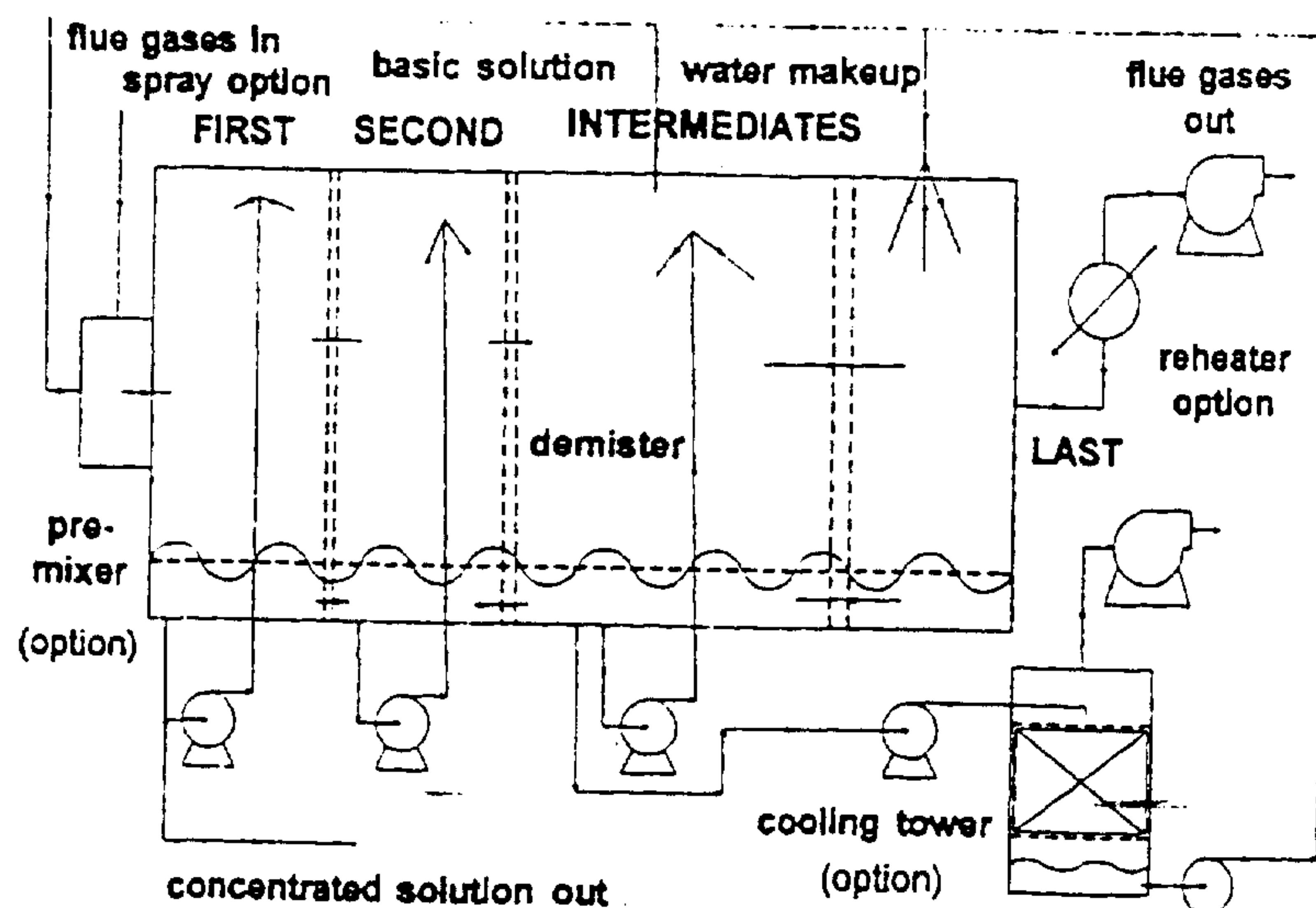
Schematic illustration of the novel scrubber
