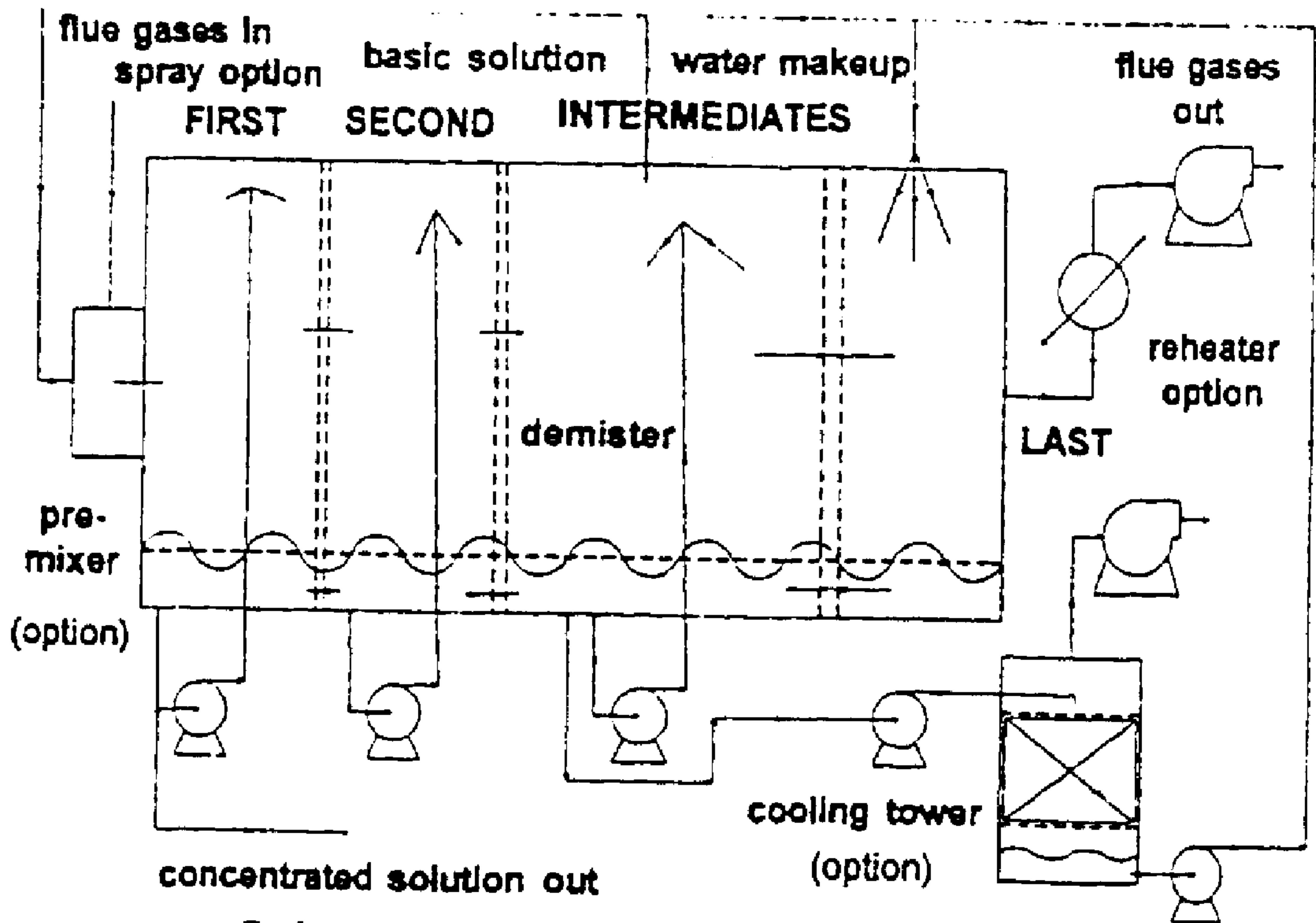
Schematic illustration of the novel scrubber
