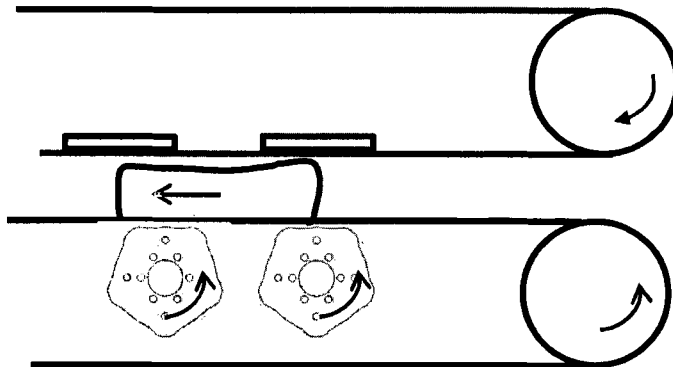
FIG. 1c (prior art)
