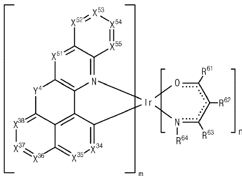
[Formula 1-15]
