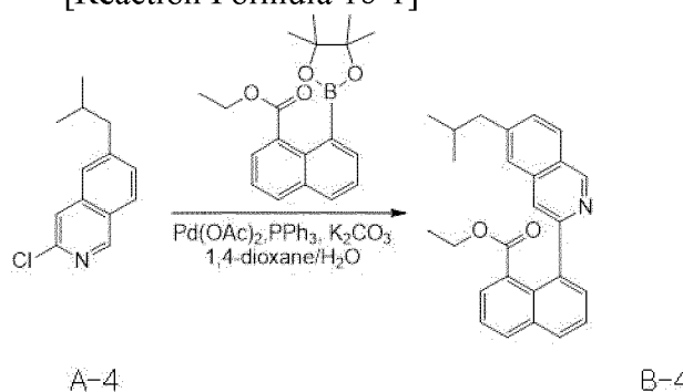
[Reaction Formula 16-1]
