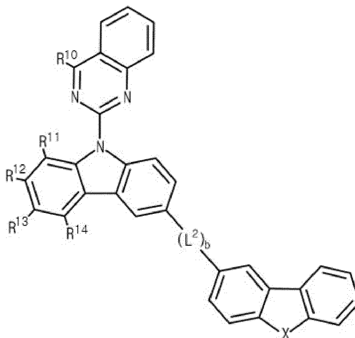
[Formula 3-2]
