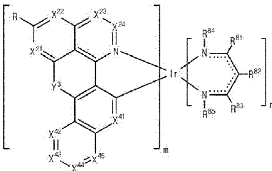
[Formula 1-22]
