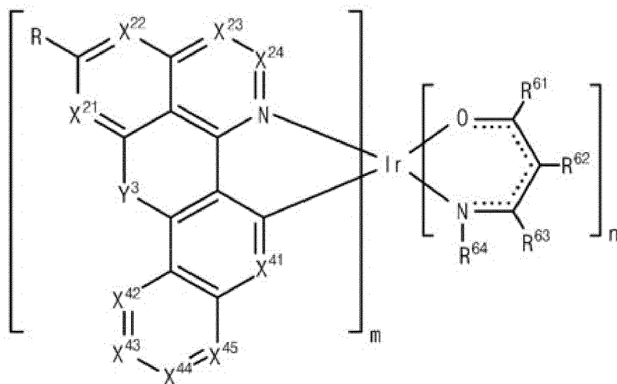
[Formula 1-13]
