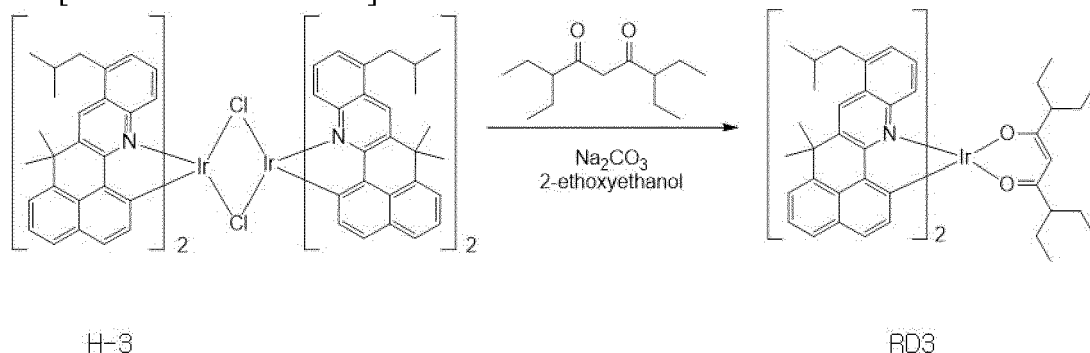
[Reaction Formula 15-8]
