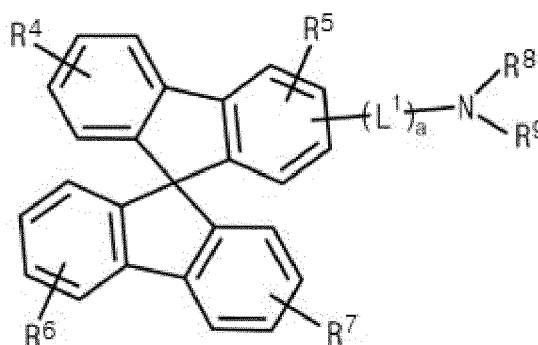
[Formula 2-1]
