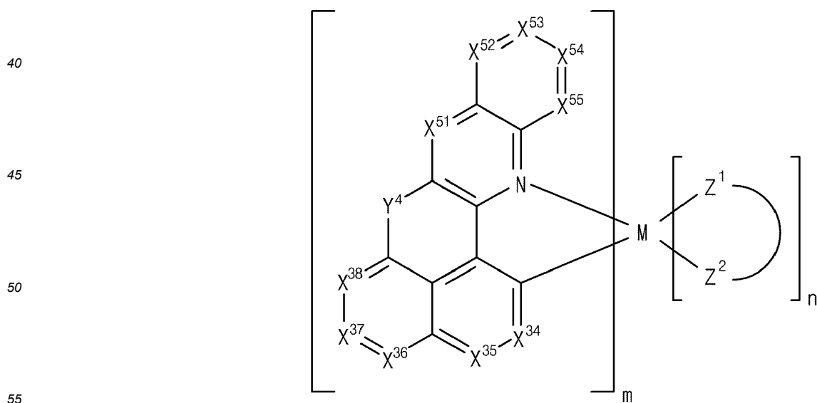
[Formula 1-6]
