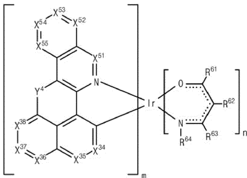
[Formula 1-15]
