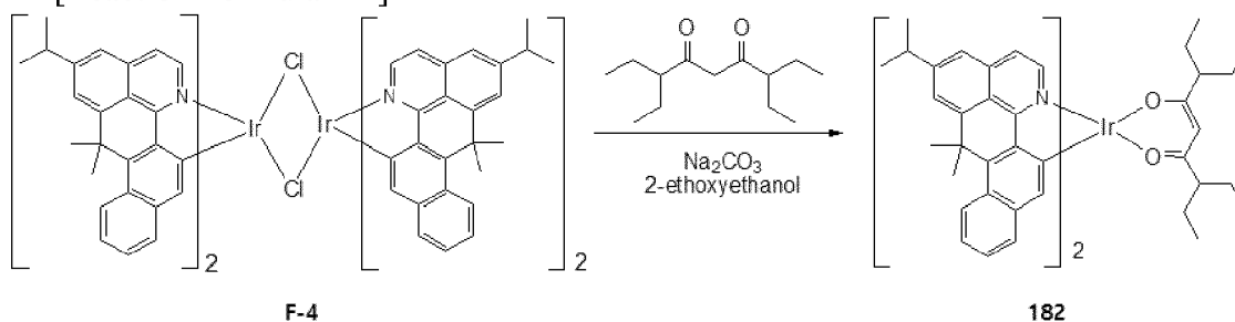
[Reaction Formula 4-5]
