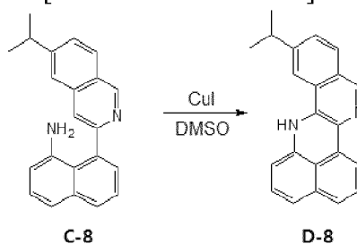
[Reaction Formula 8-2]
