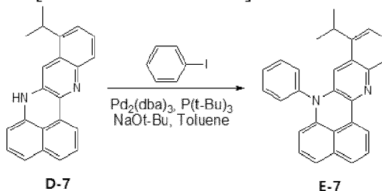
[Reaction Formula 7-3]
