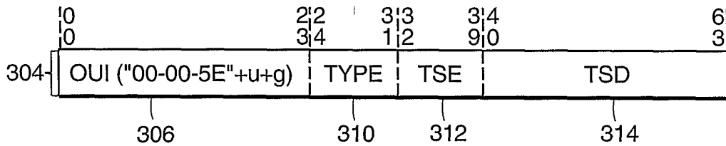
FIG. 15C INTERFACE IDENTIFIER FORMAT FOR IANA
