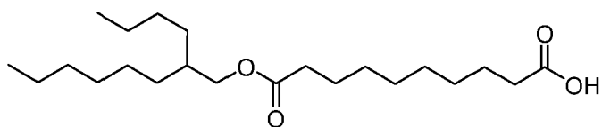
10-((2-Butyloctyl)oxy)-10-oxodecanoic acid
