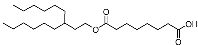
8-((3-Hexylnonyl)oxy)-8-oxooctanoic acid
