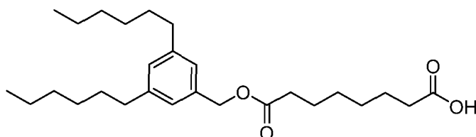
8-((3,5-Dihexylbenzyl)oxy)-8-oxooctanoic acid
