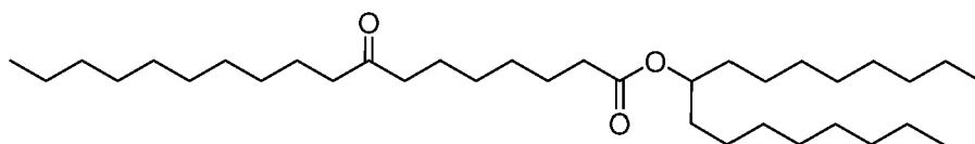
Heptadecan-9-yl 8-oxooctadecanoate
