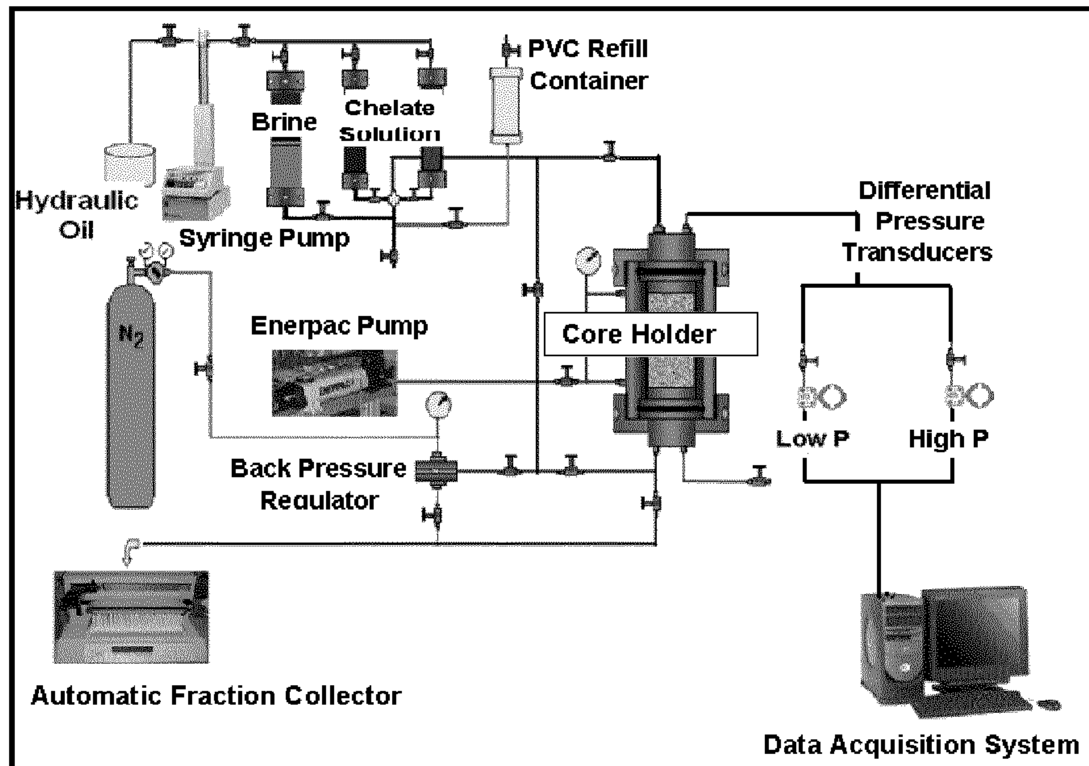
Fig. 1 - Core flooding set-up.
