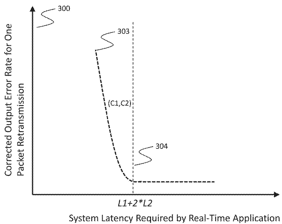
Figure 3. Combined Latency versus Output Error Rate
