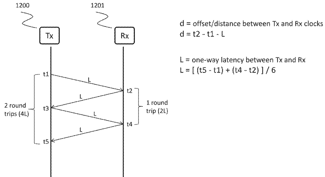
Figure 12. Transmitter/Receiver Clock synchronization Diagram
