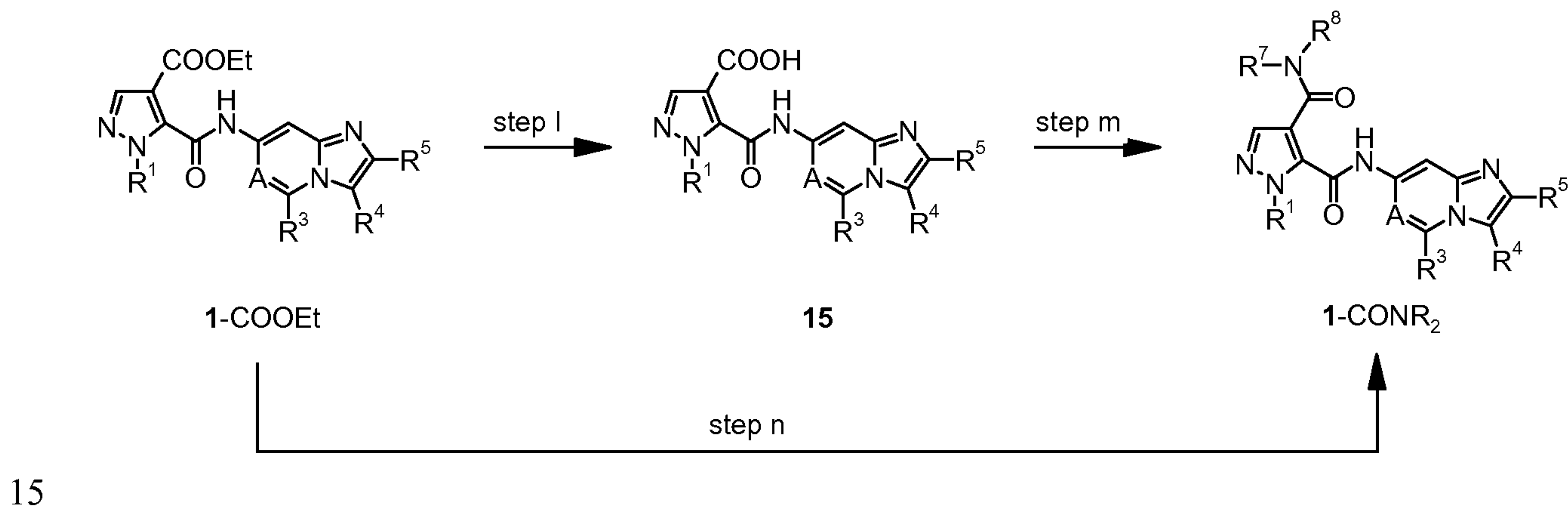
Scheme 5
