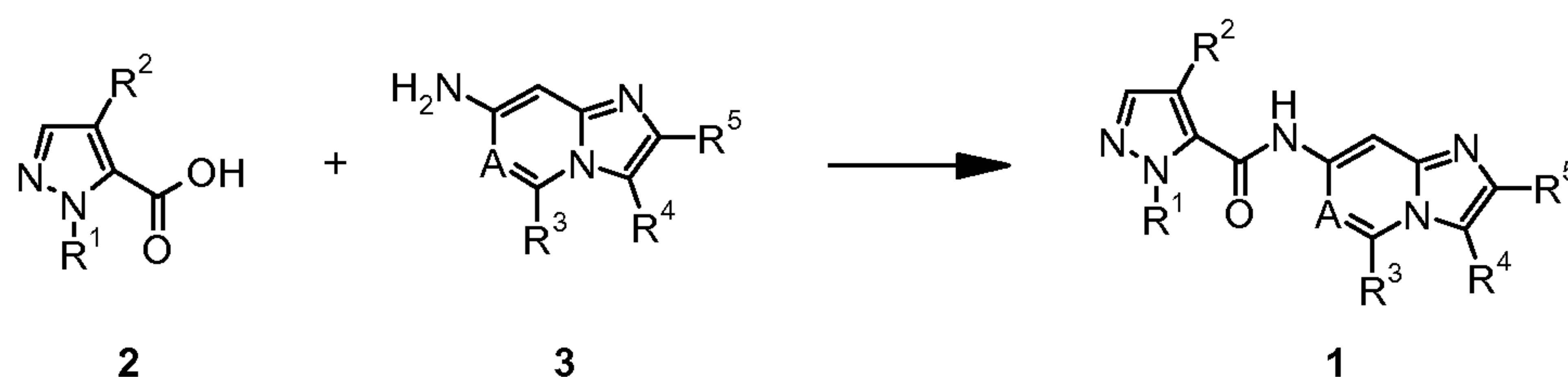
Scheme 1
