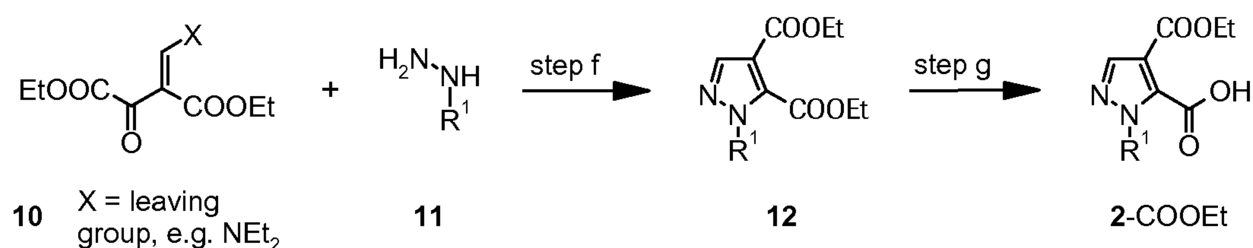
Scheme 3
