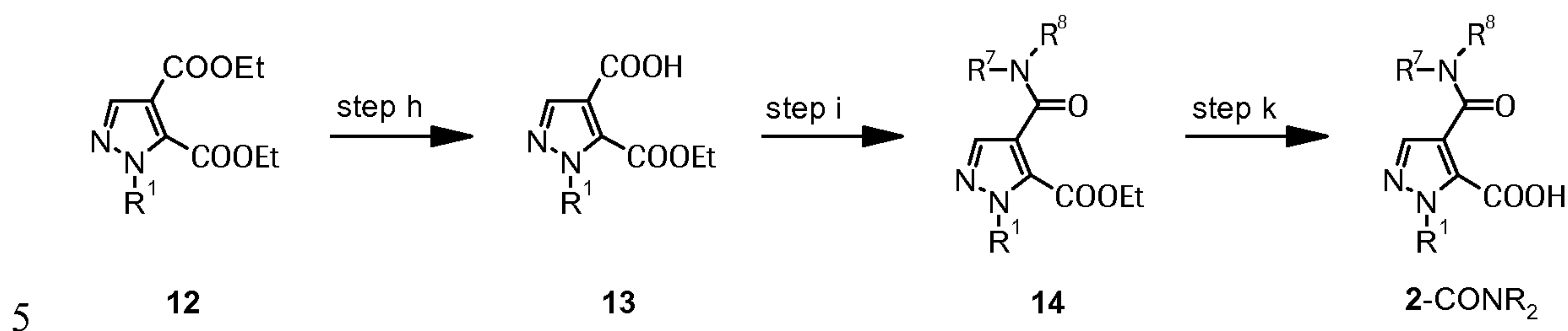
Scheme 4
