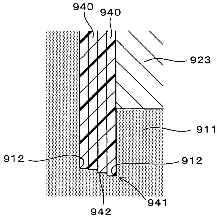
FIG. 30 RELATED ART
