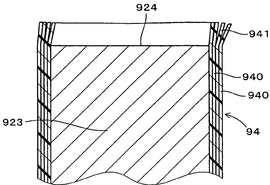
FIG. 31 RELATED ART
