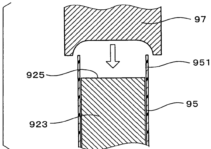
FIG. 35 RELATED ART
