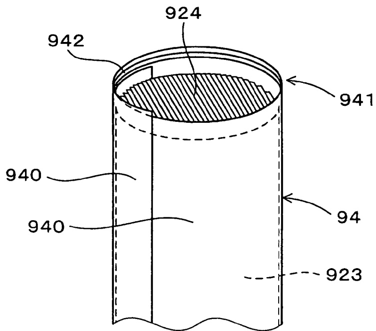
FIG. 29 RELATED ART
