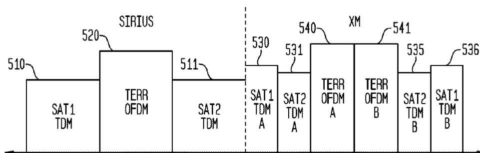
FIG. 5 SPECTRUM DIAGRAM
