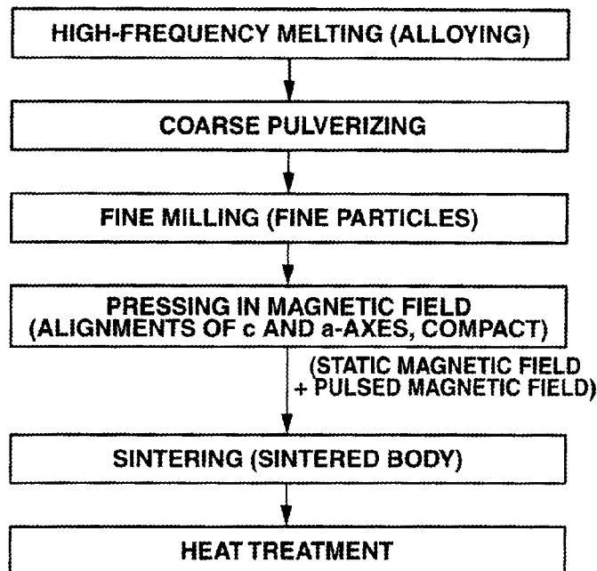
FIG.3A INVENTIVE PROCESS
