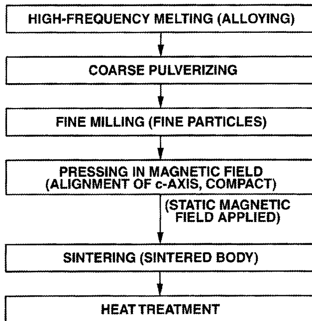
FIG.3B PRIOR ART PROCESS
